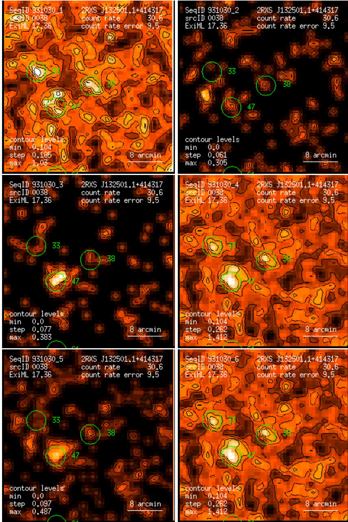
Figure 38: RASS 931030: detection 0038: band rate images, Gaussian filter: (1) PSPC channels 11 – 41, (2) 52 – 90, (3) 91 – 201, (4) 11 – 235, (5) 52 – 201, (6) 11 – 201. Broad band rates in counts/ks. Band rate contour levels in counts/ks/arcmin 2 .
