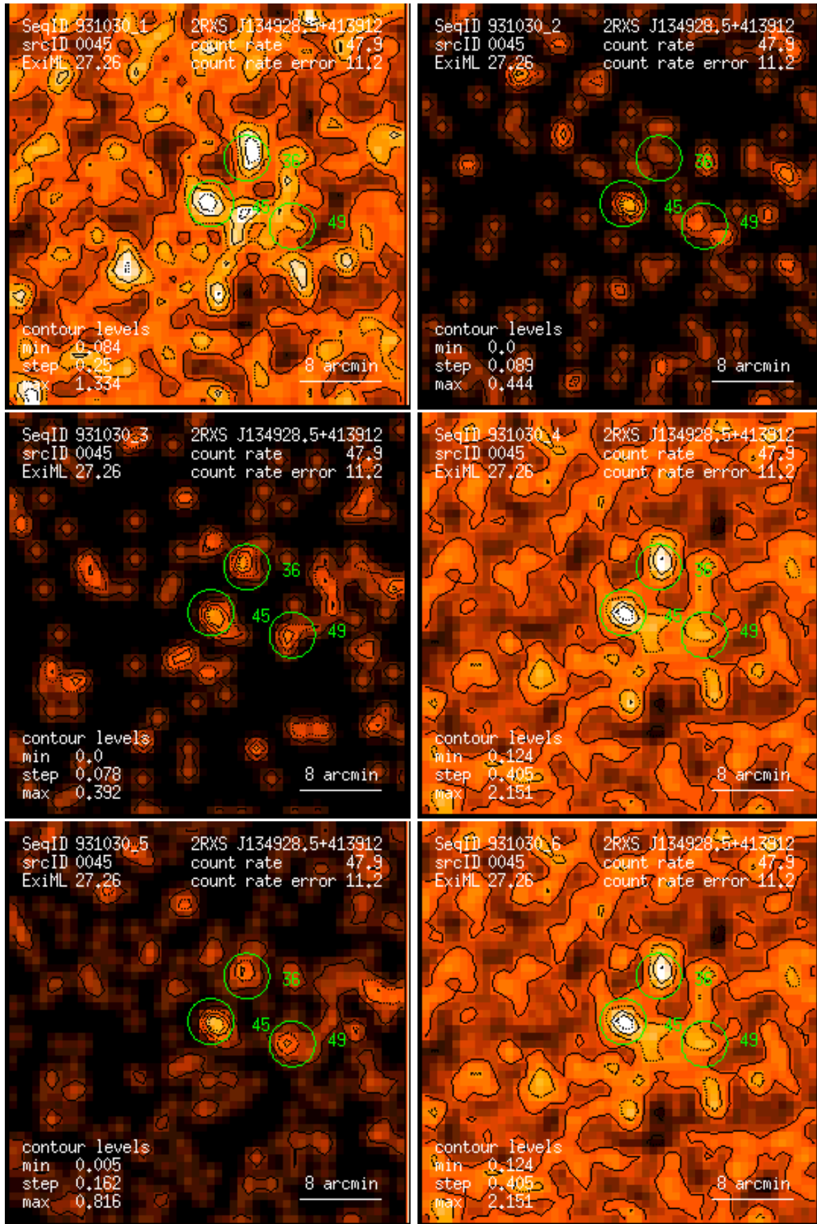
Figure 45: RASS 931030: detection 0045: band rate images, Gaussian filter: (1) PSPC channels 11 – 41, (2) 52 – 90, (3) 91 – 201, (4) 11 – 235, (5) 52 – 201, (6) 11 – 201. Broad band rates in counts/ks. Band rate contour levels in counts/ks/arcmin 2 .
