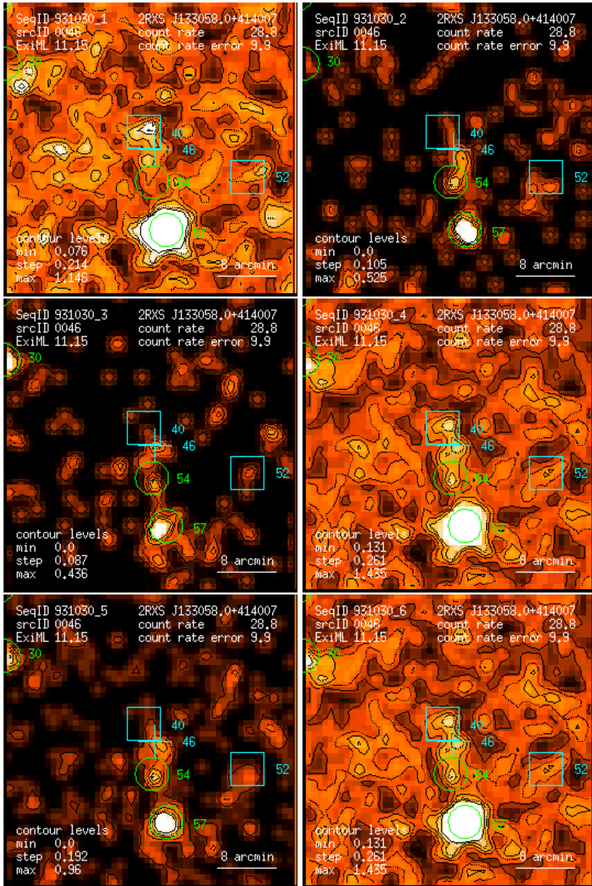
Figure 46: RASS 931030: detection 0046: band rate images, Gaussian filter: (1) PSPC channels 11 – 41, (2) 52 – 90, (3) 91 – 201, (4) 11 – 235, (5) 52 – 201, (6) 11 – 201. Broad band rates in counts/ks. Band rate contour levels in counts/ks/arcmin 2 .
