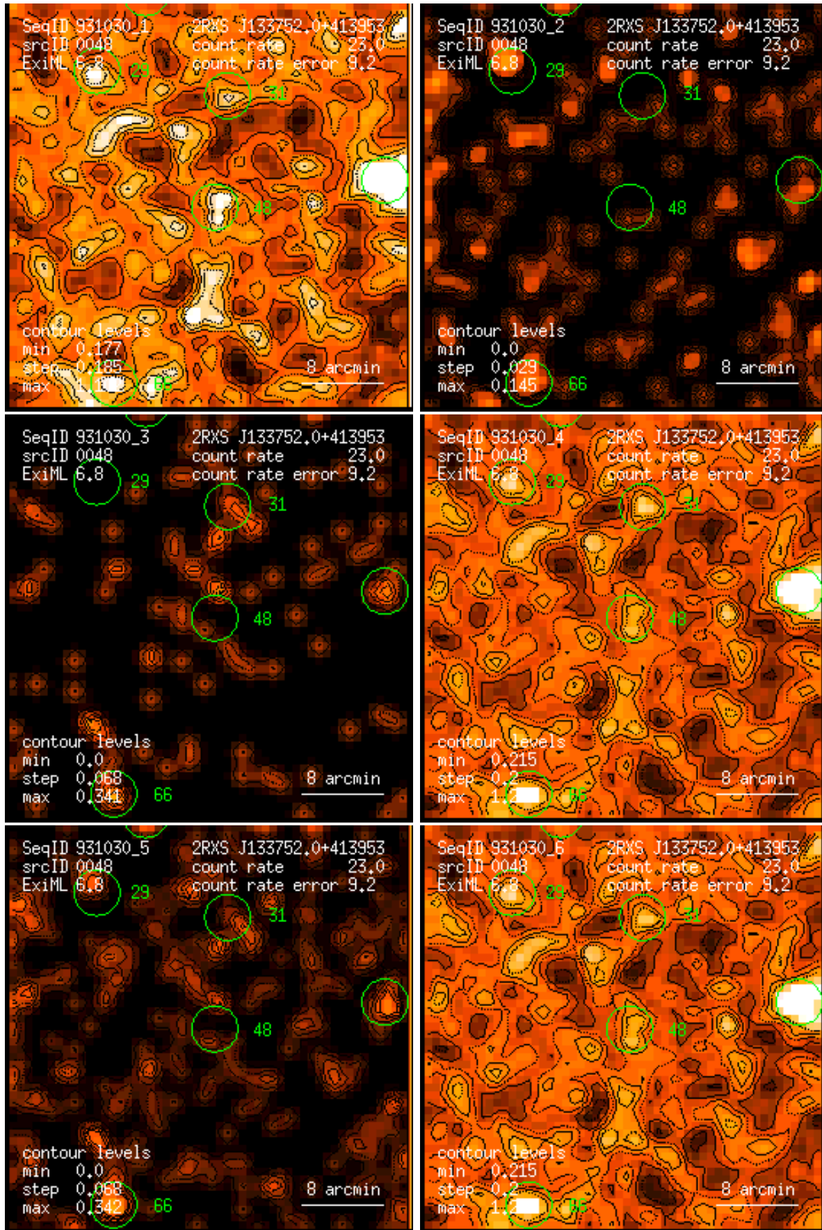
Figure 48: RASS 931030: detection 0048: band rate images, Gaussian filter: (1) PSPC channels 11 – 41, (2) 52 – 90, (3) 91 – 201, (4) 11 – 235, (5) 52 – 201, (6) 11 – 201. Broad band rates in counts/ks. Band rate contour levels in counts/ks/arcmin 2 .
