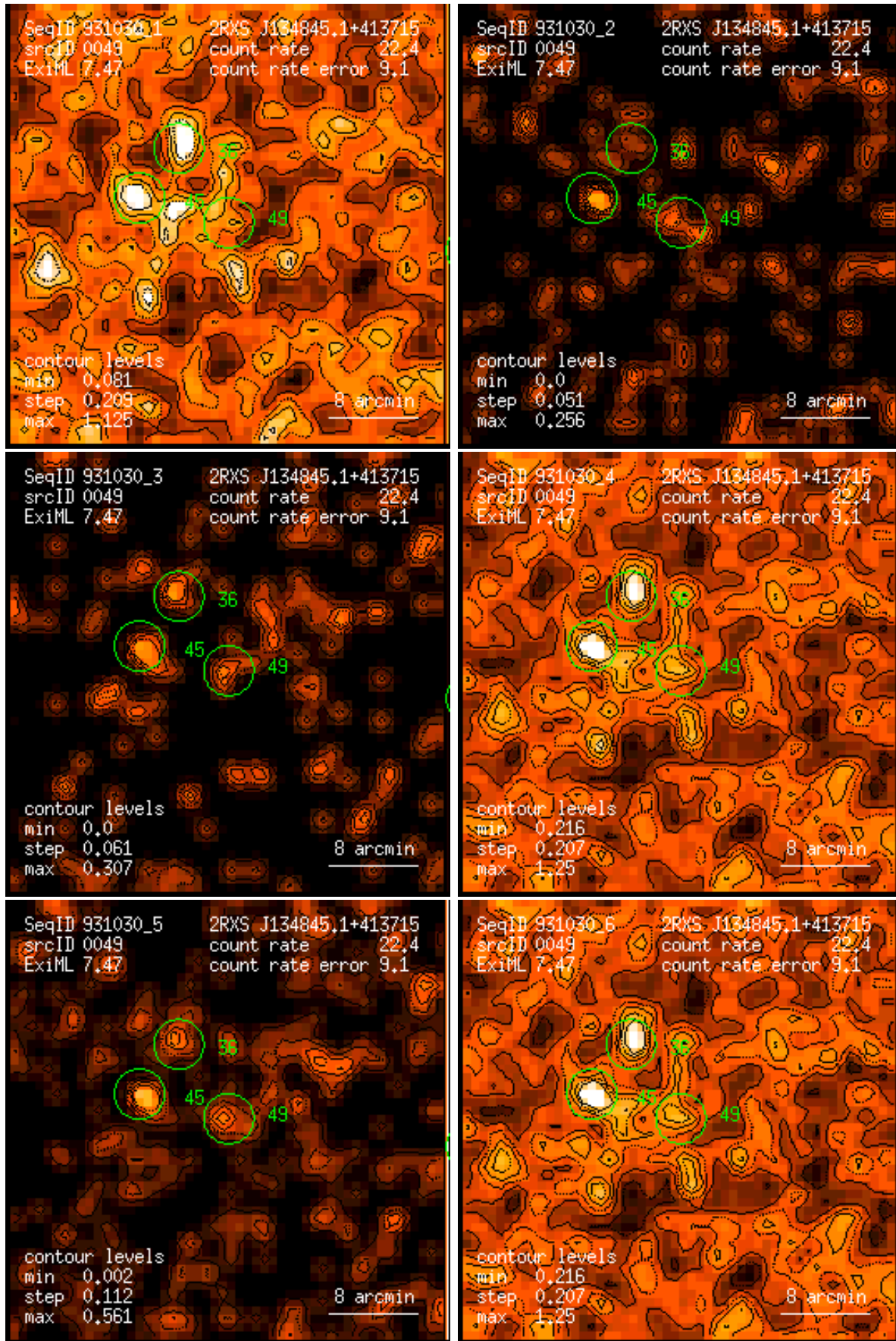
Figure 49: RASS 931030: detection 0049: band rate images, Gaussian filter: (1) PSPC channels 11 – 41, (2) 52 – 90, (3) 91 – 201, (4) 11 – 235, (5) 52 – 201, (6) 11 – 201. Broad band rates in counts/ks. Band rate contour levels in counts/ks/arcmin 2 .
