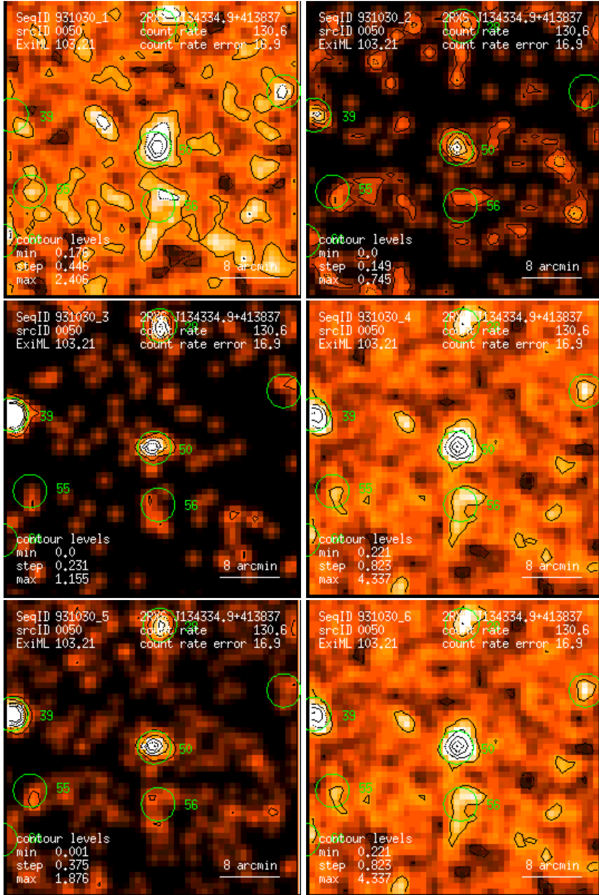
Figure 50: RASS 931030: detection 0050: band rate images, Gaussian filter: (1) PSPC channels 11 – 41, (2) 52 – 90, (3) 91 – 201, (4) 11 – 235, (5) 52 – 201, (6) 11 – 201. Broad band rates in counts/ks. Band rate contour levels in counts/ks/arcmin 2 .
