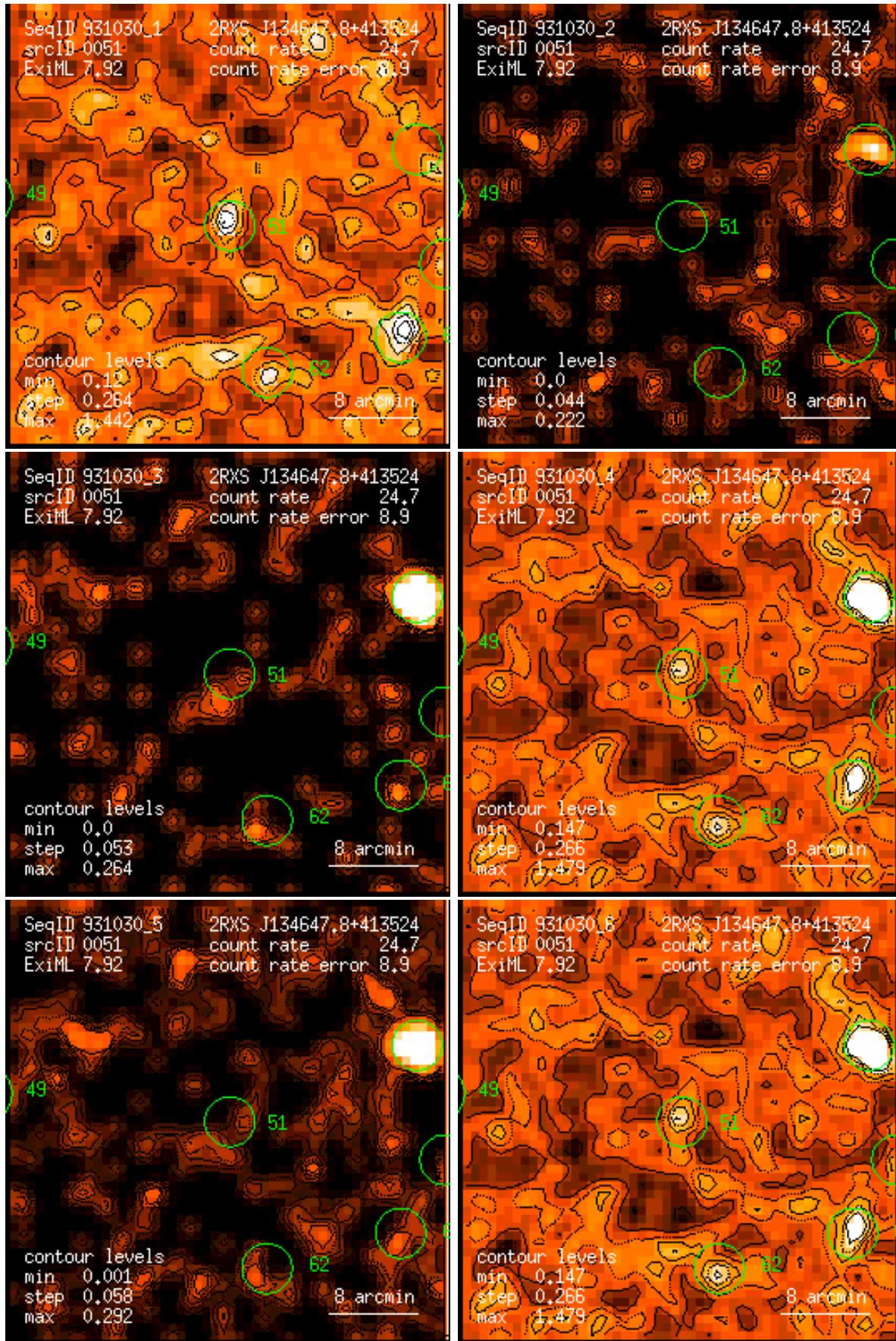
Figure 51: RASS 931030: detection 0051: band rate images, Gaussian filter: (1) PSPC channels 11 – 41, (2) 52 – 90, (3) 91 – 201, (4) 11 – 235, (5) 52 – 201, (6) 11 – 201. Broad band rates in counts/ks. Band rate contour levels in counts/ks/arcmin 2 .
