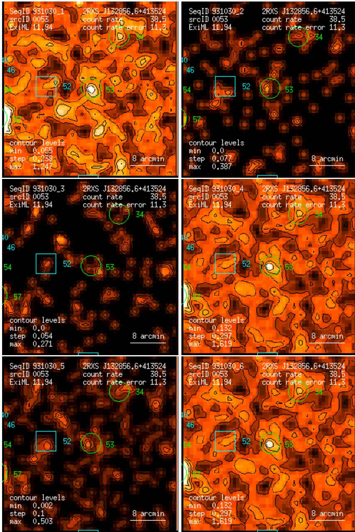
Figure 53: RASS 931030: detection 0053: band rate images, Gaussian filter: (1) PSPC channels 11 – 41, (2) 52 – 90, (3) 91 – 201, (4) 11 – 235, (5) 52 – 201, (6) 11 – 201. Broad band rates in counts/ks. Band rate contour levels in counts/ks/arcmin 2 .
