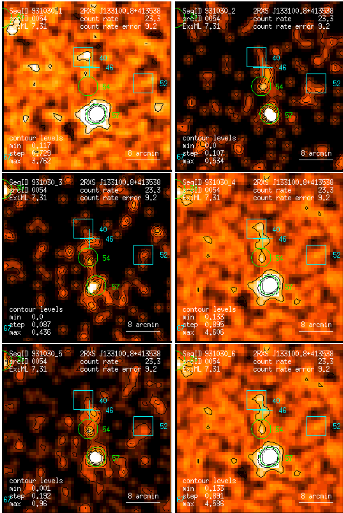
Figure 54: RASS 931030: detection 0054: band rate images, Gaussian filter: (1) PSPC channels 11 – 41, (2) 52 – 90, (3) 91 – 201, (4) 11 – 235, (5) 52 – 201, (6) 11 – 201. Broad band rates in counts/ks. Band rate contour levels in counts/ks/arcmin 2 .
