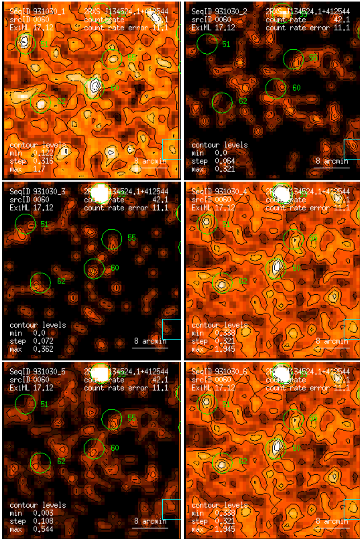
Figure 60: RASS 931030: detection 0060: band rate images, Gaussian filter: (1) PSPC channels 11 – 41, (2) 52 – 90, (3) 91 – 201, (4) 11 – 235, (5) 52 – 201, (6) 11 – 201. Broad band rates in counts/ks. Band rate contour levels in counts/ks/arcmin 2 .
