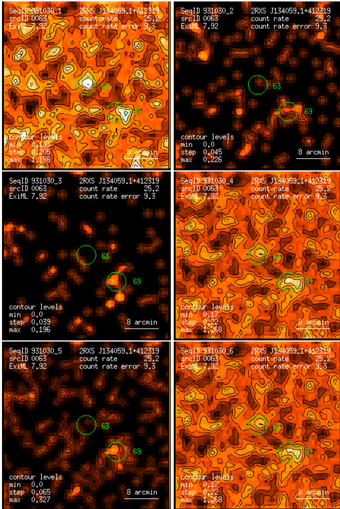
Figure 63: RASS 931030: detection 0063: band rate images, Gaussian filter: (1) PSPC channels 11 – 41, (2) 52 – 90, (3) 91 – 201, (4) 11 – 235, (5) 52 – 201, (6) 11 – 201. Broad band rates in counts/ks. Band rate contour levels in counts/ks/arcmin 2 .
