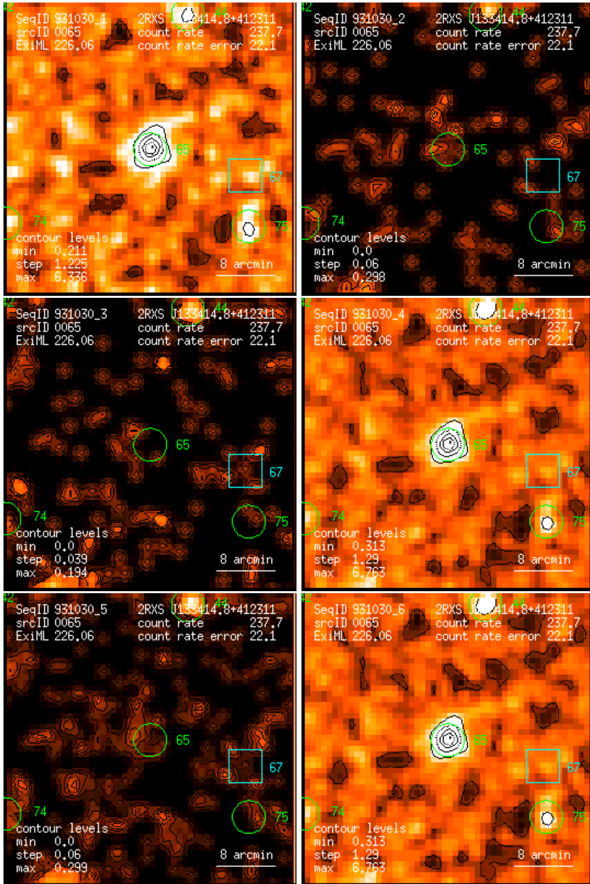
Figure 65: RASS 931030: detection 0065: band rate images, Gaussian filter: (1) PSPC channels 11 – 41, (2) 52 – 90, (3) 91 – 201, (4) 11 – 235, (5) 52 – 201, (6) 11 – 201. Broad band rates in counts/ks. Band rate contour levels in counts/ks/arcmin 2 .
