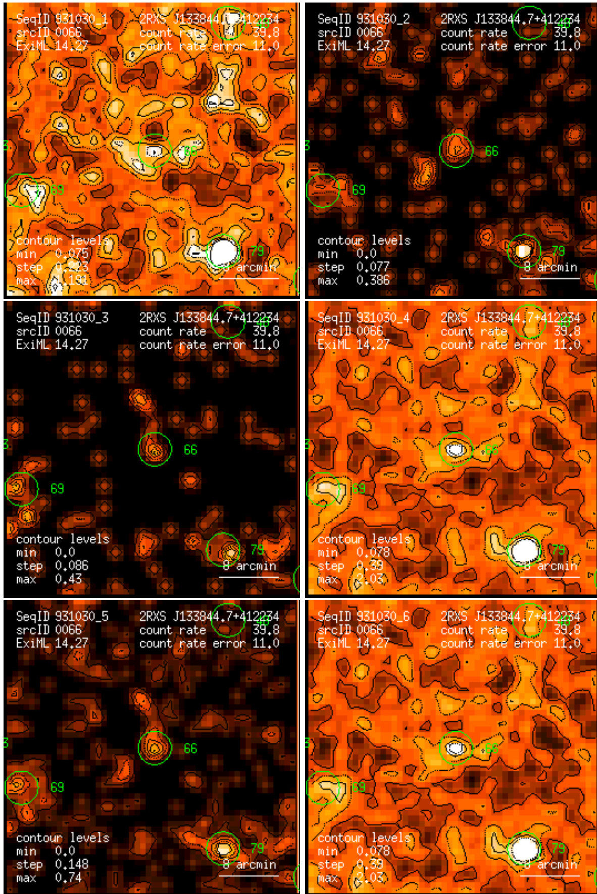
Figure 66: RASS 931030: detection 0066: band rate images, Gaussian filter: (1) PSPC channels 11 – 41, (2) 52 – 90, (3) 91 – 201, (4) 11 – 235, (5) 52 – 201, (6) 11 – 201. Broad band rates in counts/ks. Band rate contour levels in counts/ks/arcmin 2 .
