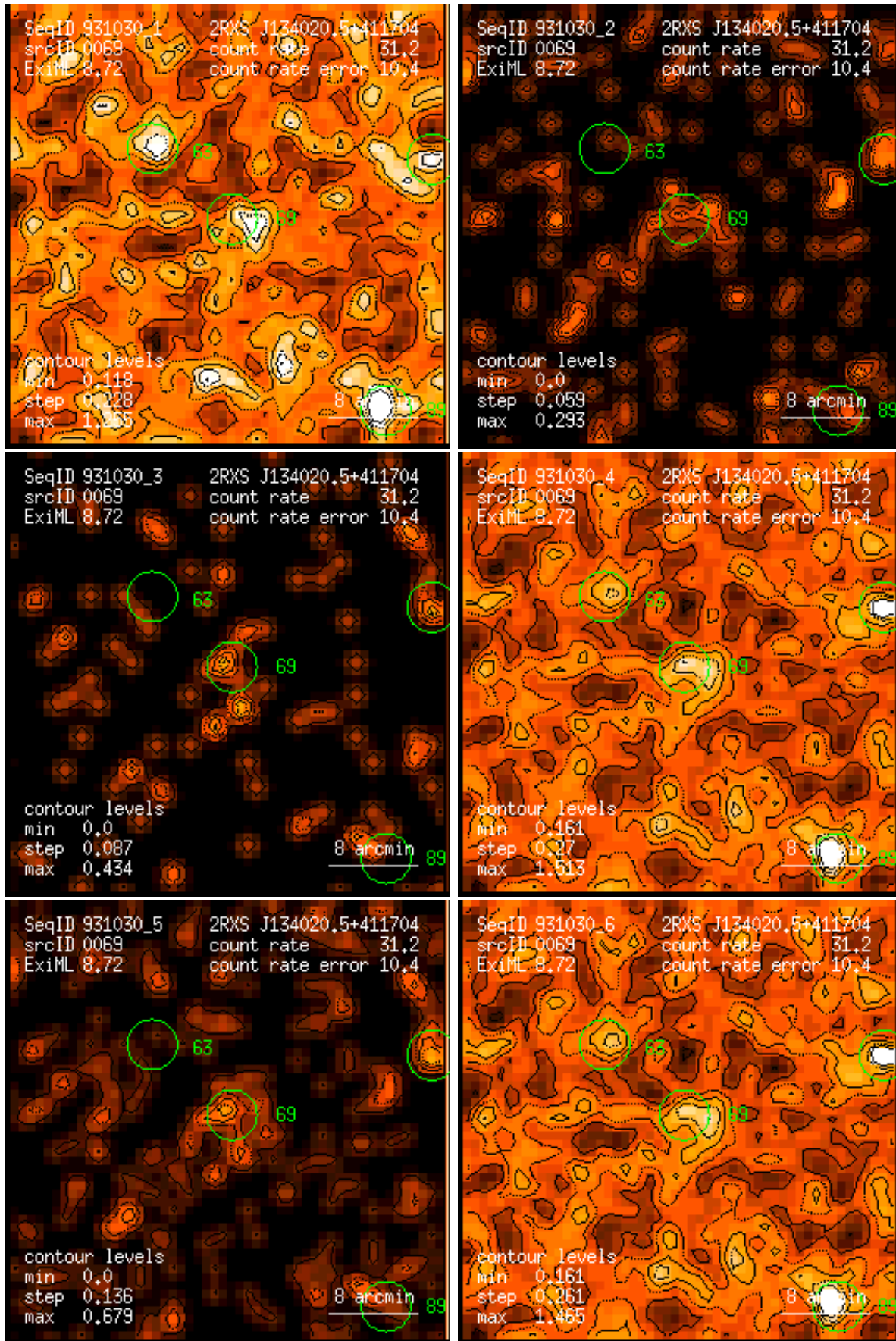
Figure 69: RASS 931030: detection 0069: band rate images, Gaussian filter: (1) PSPC channels 11 – 41, (2) 52 – 90, (3) 91 – 201, (4) 11 – 235, (5) 52 – 201, (6) 11 – 201. Broad band rates in counts/ks. Band rate contour levels in counts/ks/arcmin 2 .
