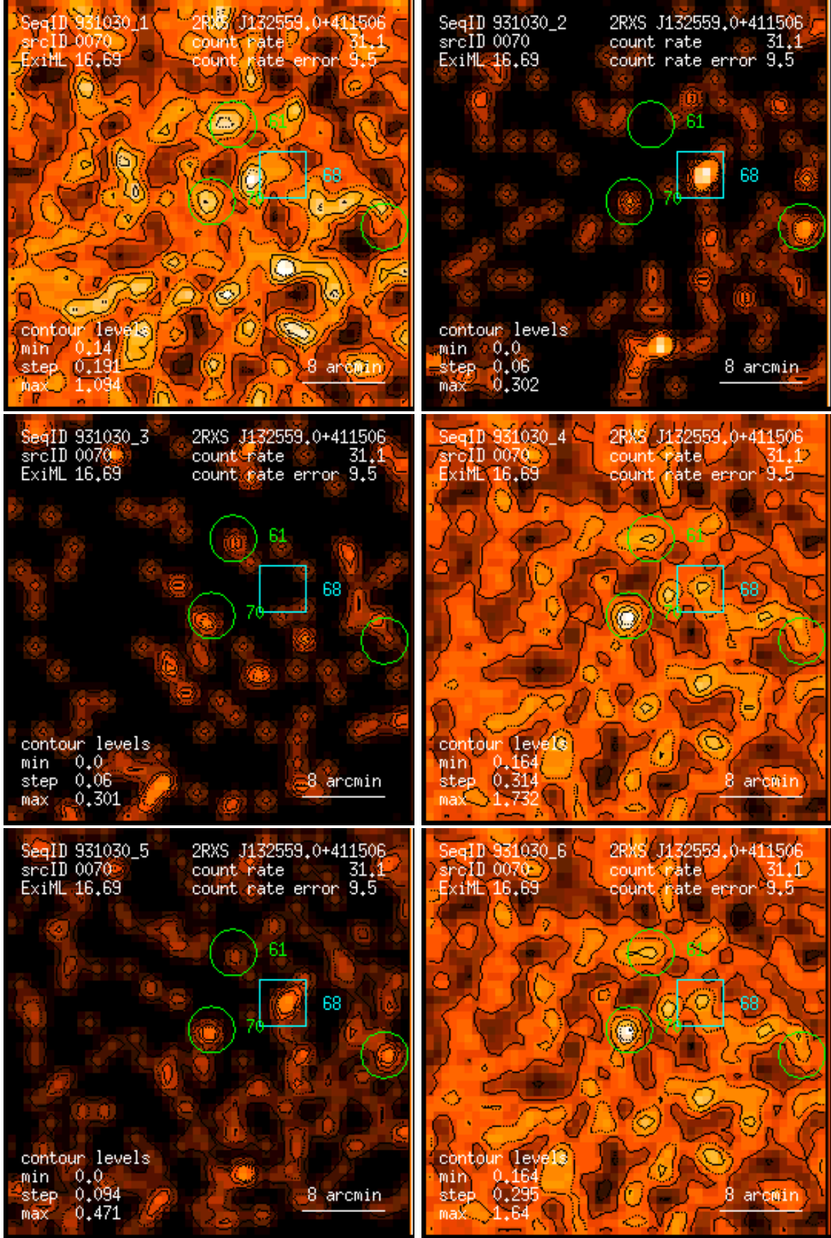
Figure 70: RASS 931030: detection 0070: band rate images, Gaussian filter: (1) PSPC channels 11 – 41, (2) 52 – 90, (3) 91 – 201, (4) 11 – 235, (5) 52 – 201, (6) 11 – 201. Broad band rates in counts/ks. Band rate contour levels in counts/ks/arcmin 2 .
