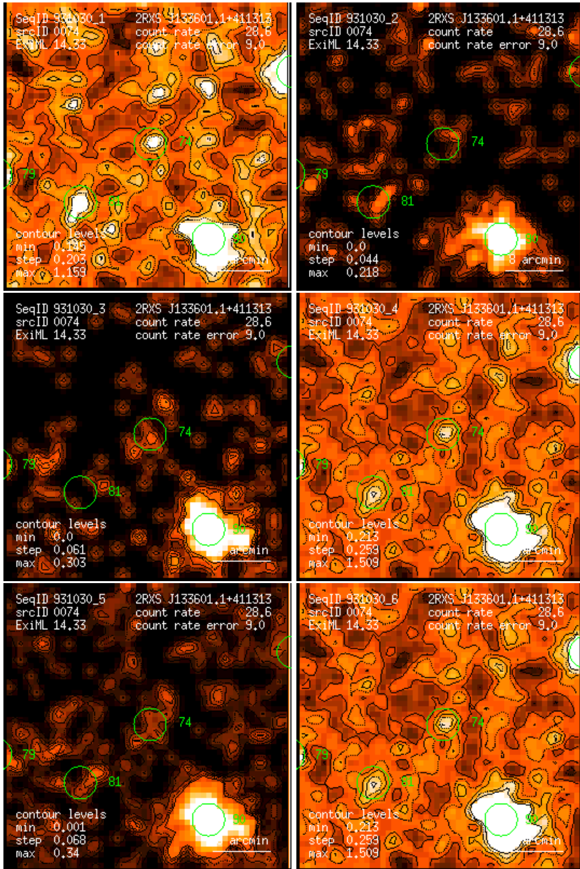
Figure 74: RASS 931030: detection 0074: band rate images, Gaussian filter: (1) PSPC channels 11 – 41, (2) 52 – 90, (3) 91 – 201, (4) 11 – 235, (5) 52 – 201, (6) 11 – 201. Broad band rates in counts/ks. Band rate contour levels in counts/ks/arcmin 2 .
