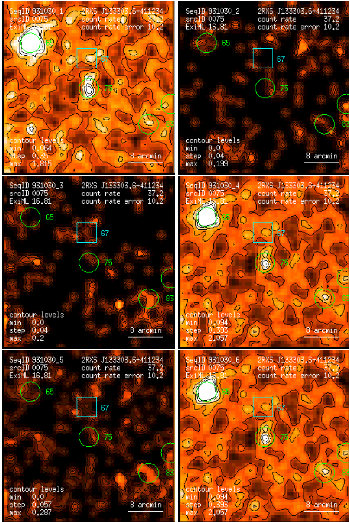
Figure 75: RASS 931030: detection 0075: band rate images, Gaussian filter: (1) PSPC channels 11 – 41, (2) 52 – 90, (3) 91 – 201, (4) 11 – 235, (5) 52 – 201, (6) 11 – 201. Broad band rates in counts/ks. Band rate contour levels in counts/ks/arcmin 2 .
