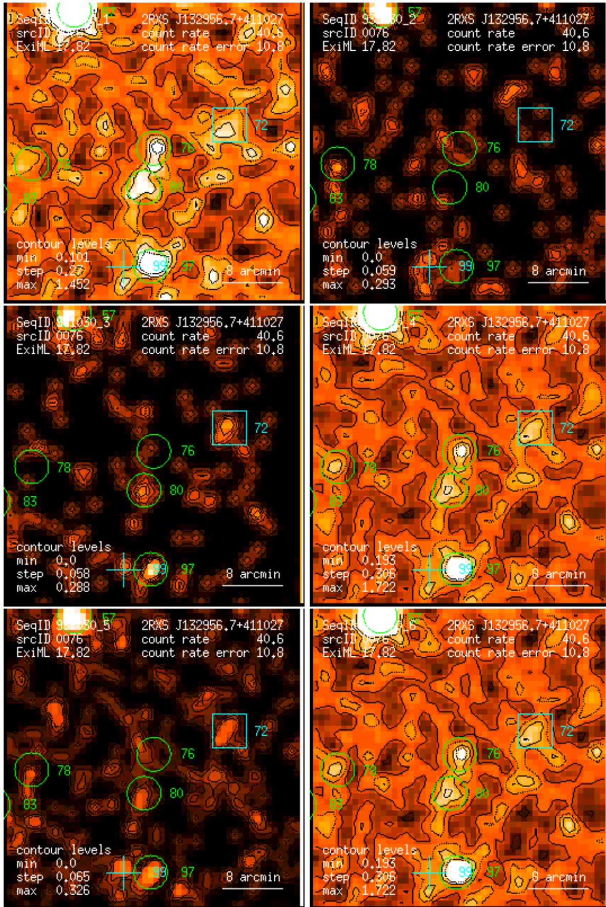
Figure 76: RASS 931030: detection 0076: band rate images, Gaussian filter: (1) PSPC channels 11 – 41, (2) 52 – 90, (3) 91 – 201, (4) 11 – 235, (5) 52 – 201, (6) 11 – 201. Broad band rates in counts/ks. Band rate contour levels in counts/ks/arcmin 2 .
