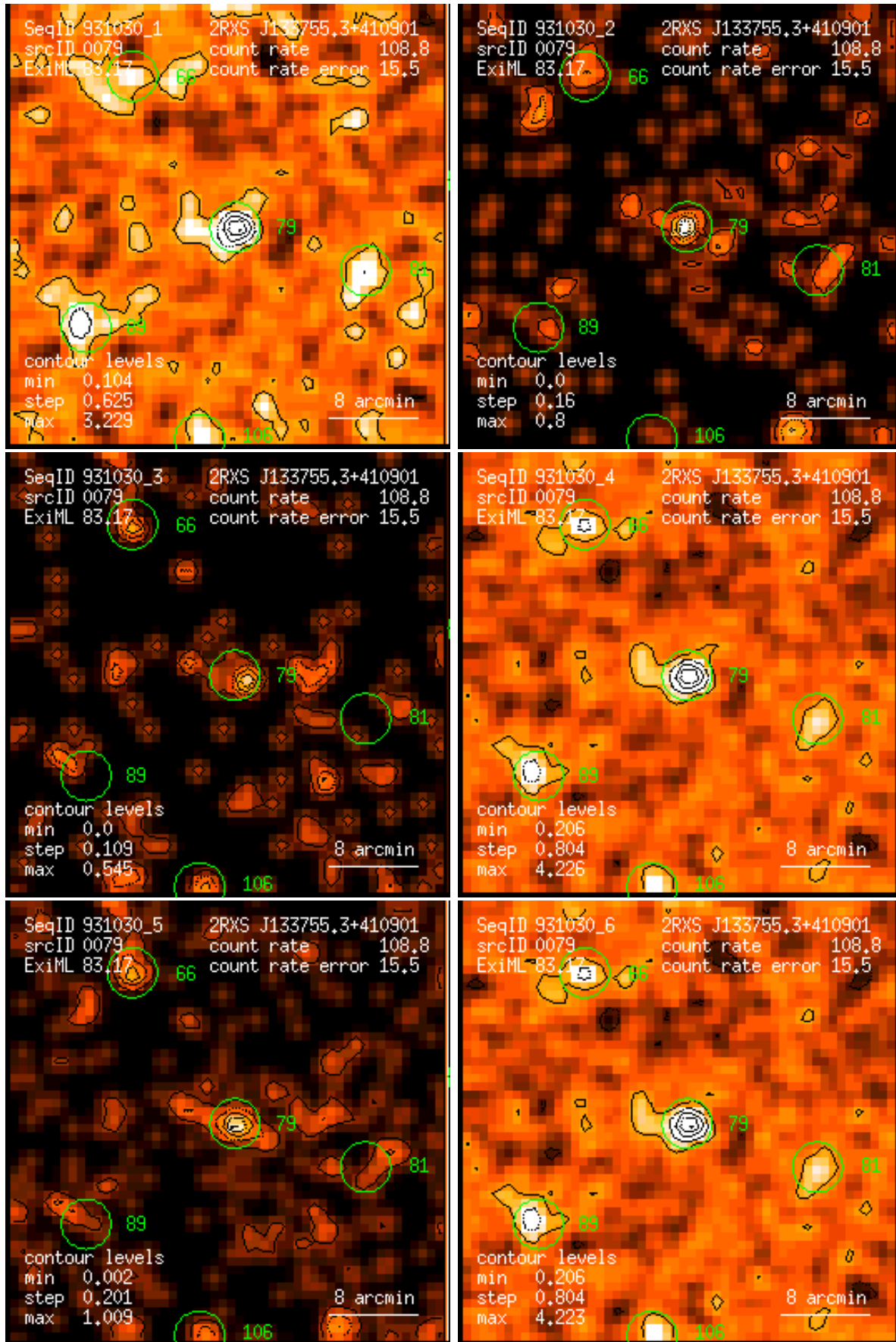
Figure 79: RASS 931030: detection 0079: band rate images, Gaussian filter: (1) PSPC channels 11 – 41, (2) 52 – 90, (3) 91 – 201, (4) 11 – 235, (5) 52 – 201, (6) 11 – 201. Broad band rates in counts/ks. Band rate contour levels in counts/ks/arcmin 2 .
