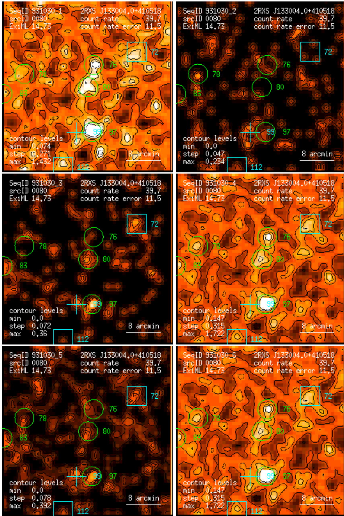
Figure 80: RASS 931030: detection 0080: band rate images, Gaussian filter: (1) PSPC channels 11 – 41, (2) 52 – 90, (3) 91 – 201, (4) 11 – 235, (5) 52 – 201, (6) 11 – 201. Broad band rates in counts/ks. Band rate contour levels in counts/ks/arcmin 2 .
