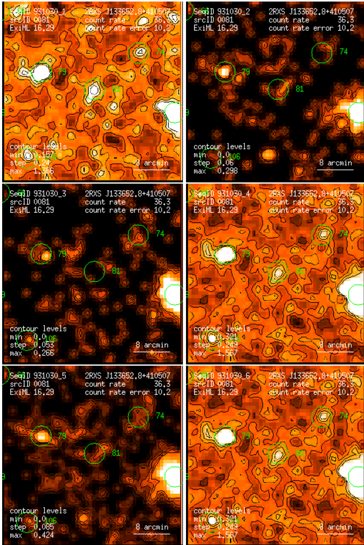
Figure 81: RASS 931030: detection 0081: band rate images, Gaussian filter: (1) PSPC channels 11 – 41, (2) 52 – 90, (3) 91 – 201, (4) 11 – 235, (5) 52 – 201, (6) 11 – 201. Broad band rates in counts/ks. Band rate contour levels in counts/ks/arcmin 2 .
