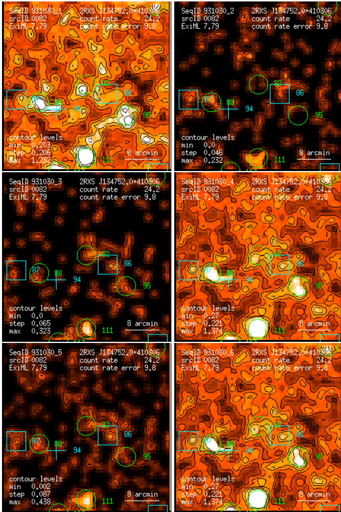
Figure 82: RASS 931030: detection 0082: band rate images, Gaussian filter: (1) PSPC channels 11 – 41, (2) 52 – 90, (3) 91 – 201, (4) 11 – 235, (5) 52 – 201, (6) 11 – 201. Broad band rates in counts/ks. Band rate contour levels in counts/ks/arcmin 2 .
