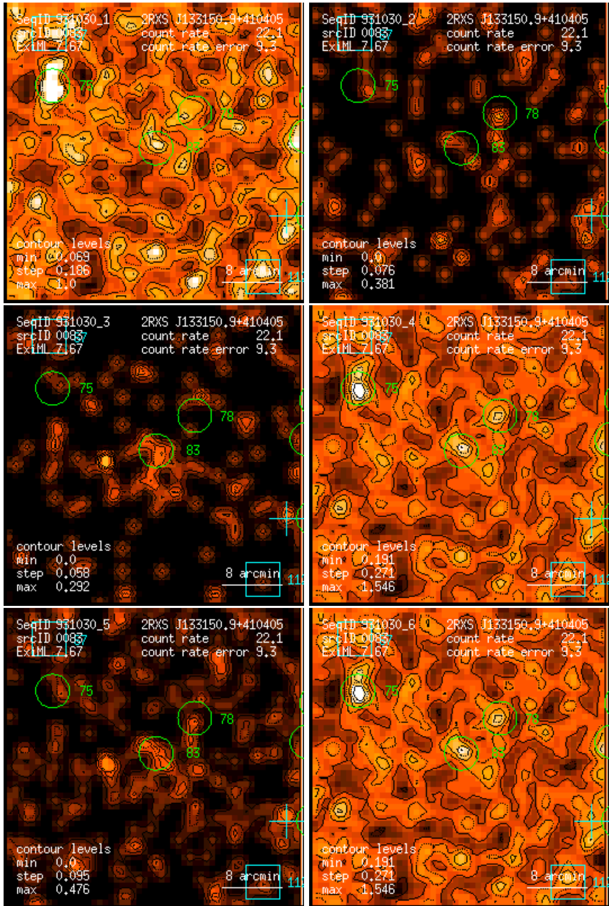
Figure 83: RASS 931030: detection 0083: band rate images, Gaussian filter: (1) PSPC channels 11 – 41, (2) 52 – 90, (3) 91 – 201, (4) 11 – 235, (5) 52 – 201, (6) 11 – 201. Broad band rates in counts/ks. Band rate contour levels in counts/ks/arcmin 2 .
