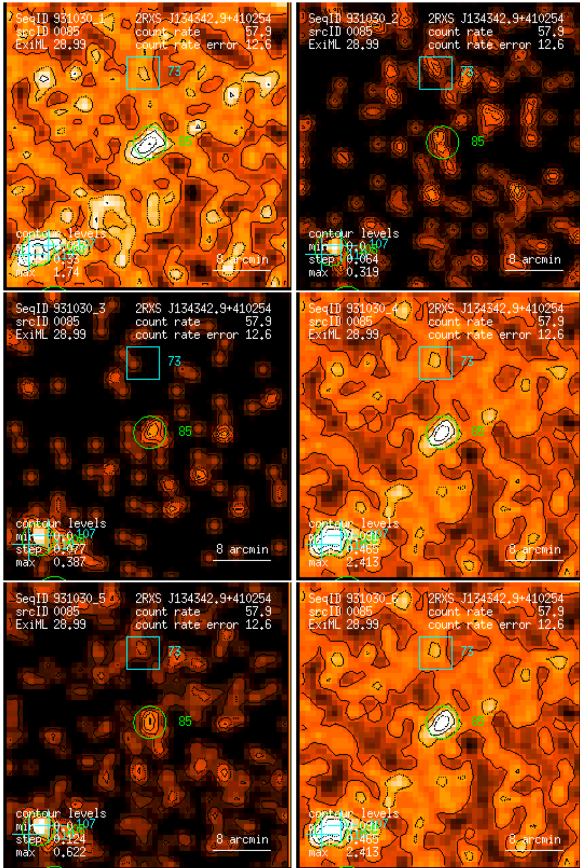
Figure 85: RASS 931030: detection 0085: band rate images, Gaussian filter: (1) PSPC channels 11 – 41, (2) 52 – 90, (3) 91 – 201, (4) 11 – 235, (5) 52 – 201, (6) 11 – 201. Broad band rates in counts/ks. Band rate contour levels in counts/ks/arcmin 2 .
