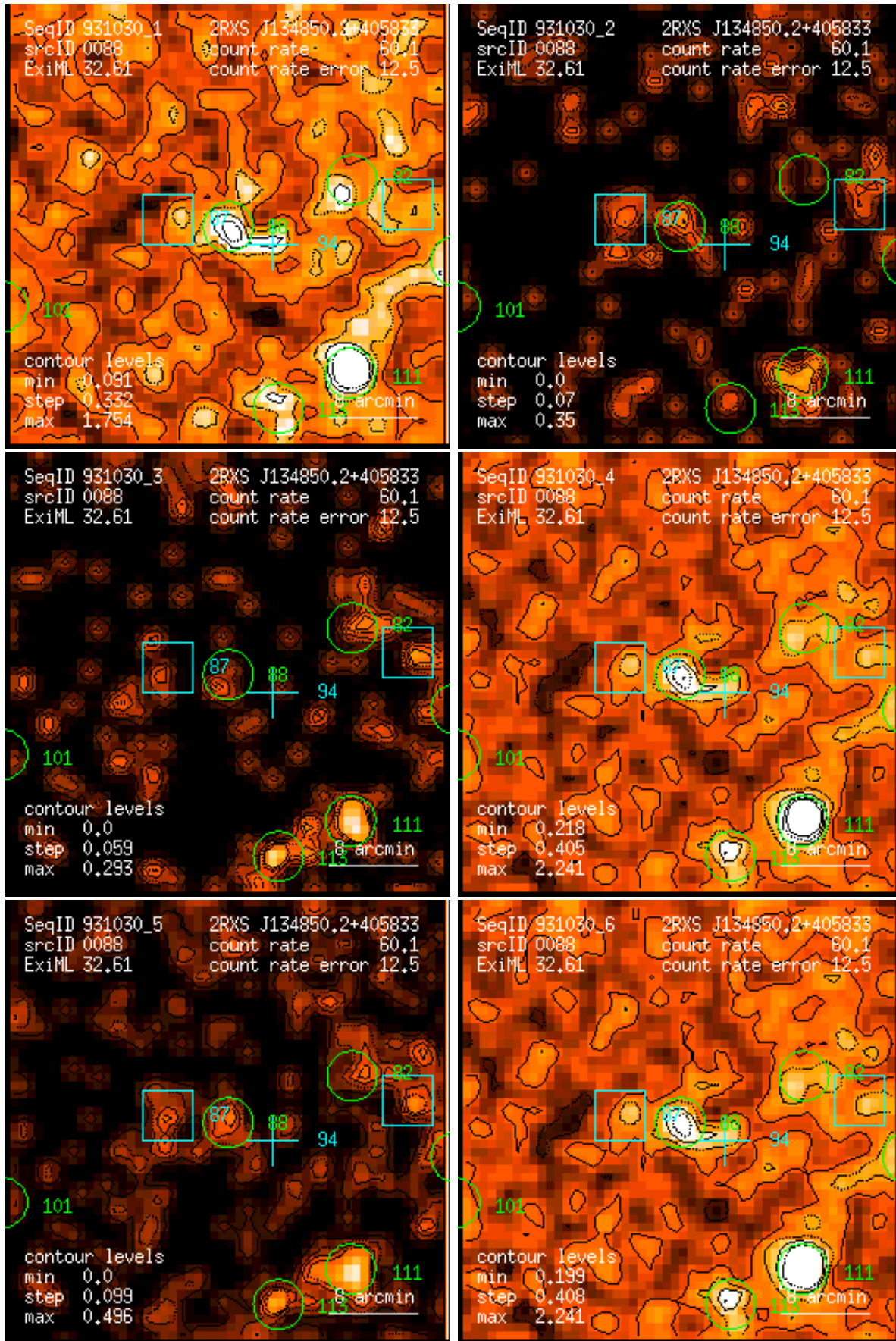
Figure 88: RASS 931030: detection 0088: band rate images, Gaussian filter: (1) PSPC channels 11 – 41, (2) 52 – 90, (3) 91 – 201, (4) 11 – 235, (5) 52 – 201, (6) 11 – 201. Broad band rates in counts/ks. Band rate contour levels in counts/ks/arcmin 2 .
