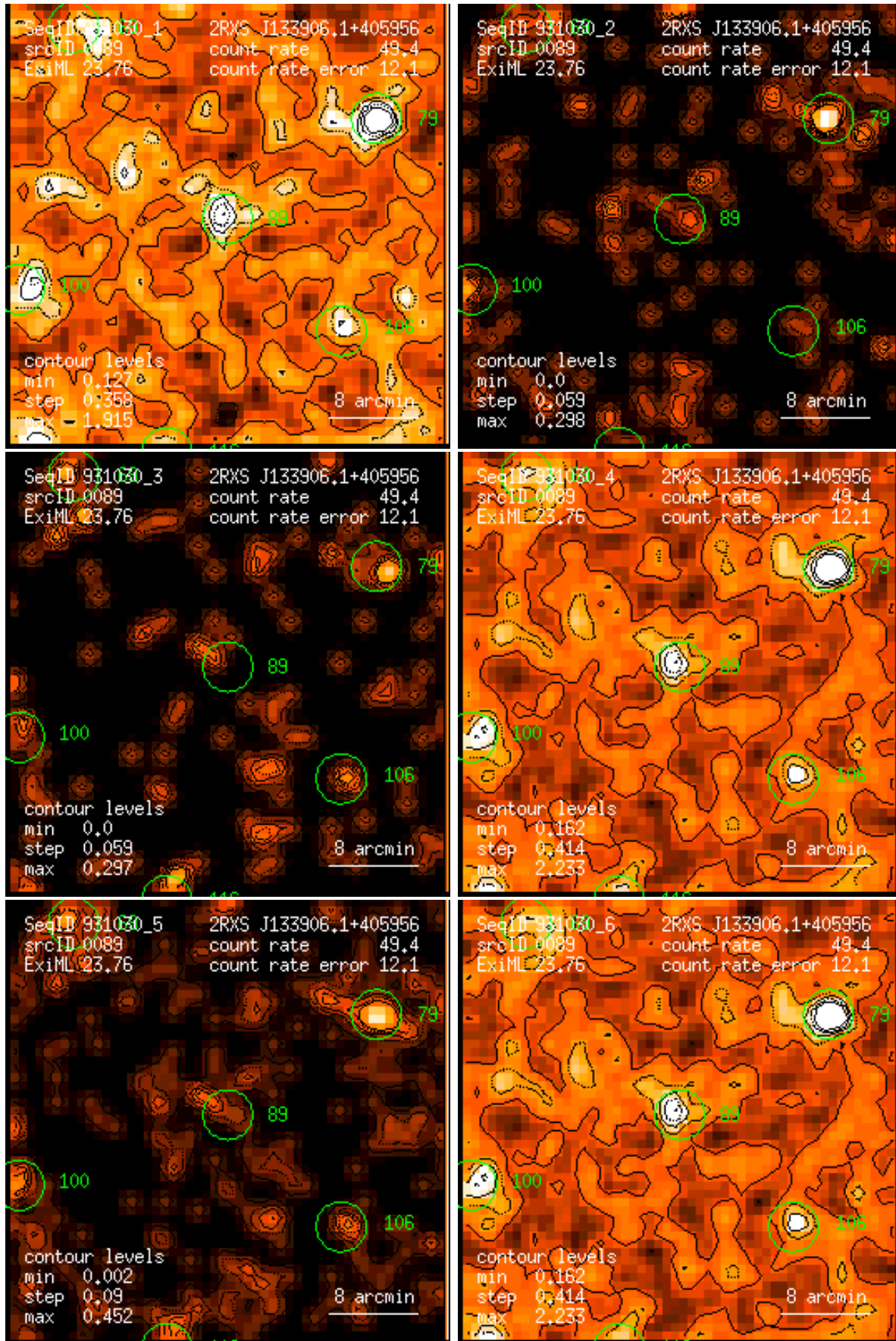
Figure 89: RASS 931030: detection 0089: band rate images, Gaussian filter: (1) PSPC channels 11 – 41, (2) 52 – 90, (3) 91 – 201, (4) 11 – 235, (5) 52 – 201, (6) 11 – 201. Broad band rates in counts/ks. Band rate contour levels in counts/ks/arcmin 2 .
