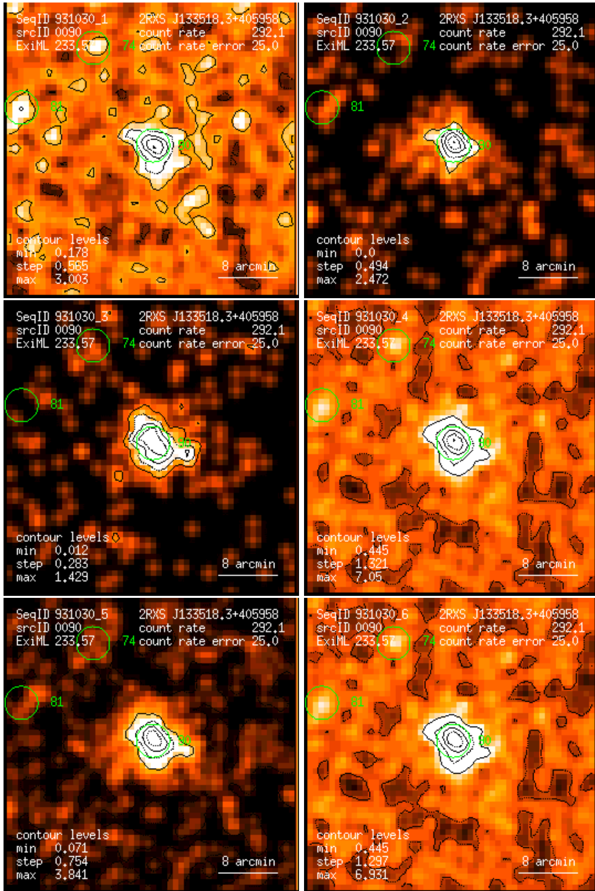
Figure 90: RASS 931030: detection 0090: band rate images, Gaussian filter: (1) PSPC channels 11 – 41, (2) 52 – 90, (3) 91 – 201, (4) 11 – 235, (5) 52 – 201, (6) 11 – 201. Broad band rates in counts/ks. Band rate contour levels in counts/ks/arcmin 2 .
