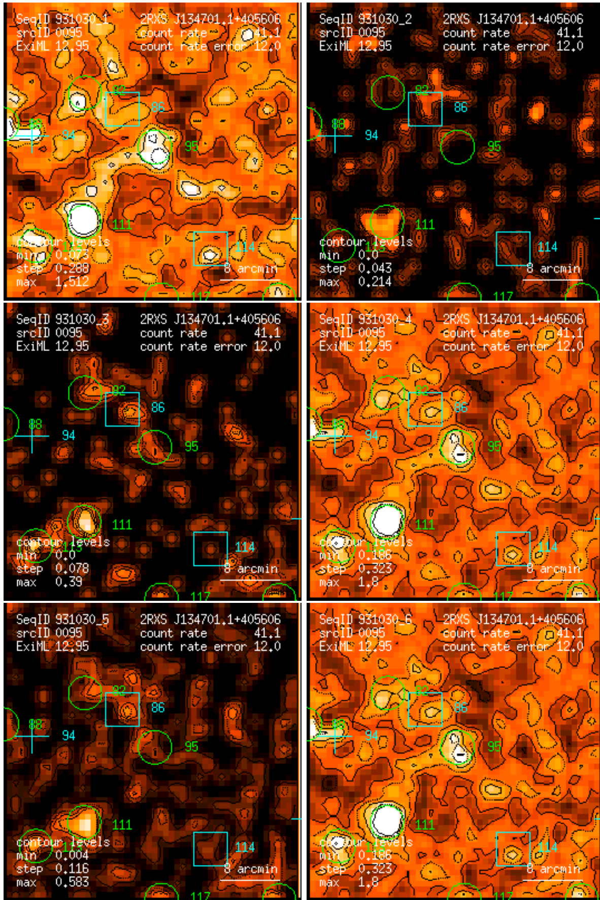
Figure 95: RASS 931030: detection 0095: band rate images, Gaussian filter: (1) PSPC channels 11 – 41, (2) 52 – 90, (3) 91 – 201, (4) 11 – 235, (5) 52 – 201, (6) 11 – 201. Broad band rates in counts/ks. Band rate contour levels in counts/ks/arcmin 2 .
