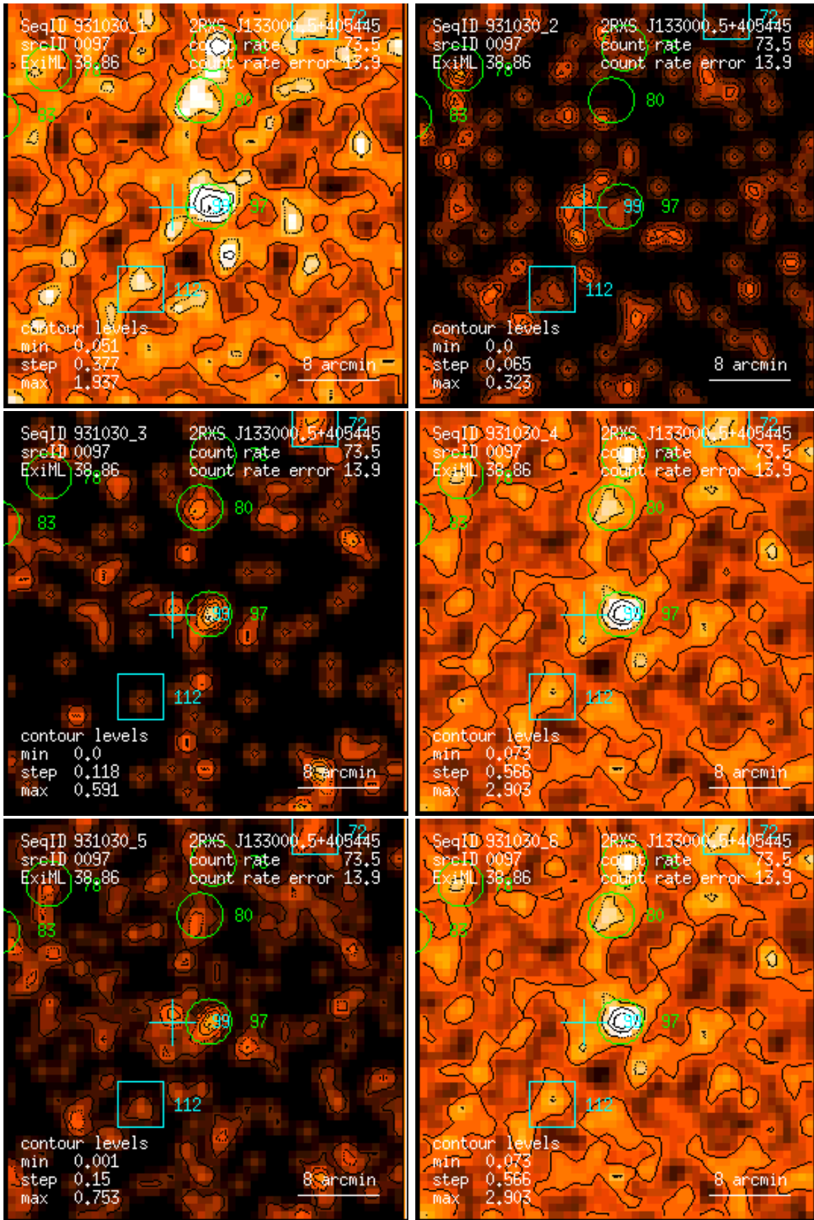
Figure 97: RASS 931030: detection 0097: band rate images, Gaussian filter: (1) PSPC channels 11 – 41, (2) 52 – 90, (3) 91 – 201, (4) 11 – 235, (5) 52 – 201, (6) 11 – 201. Broad band rates in counts/ks. Band rate contour levels in counts/ks/arcmin 2 .
