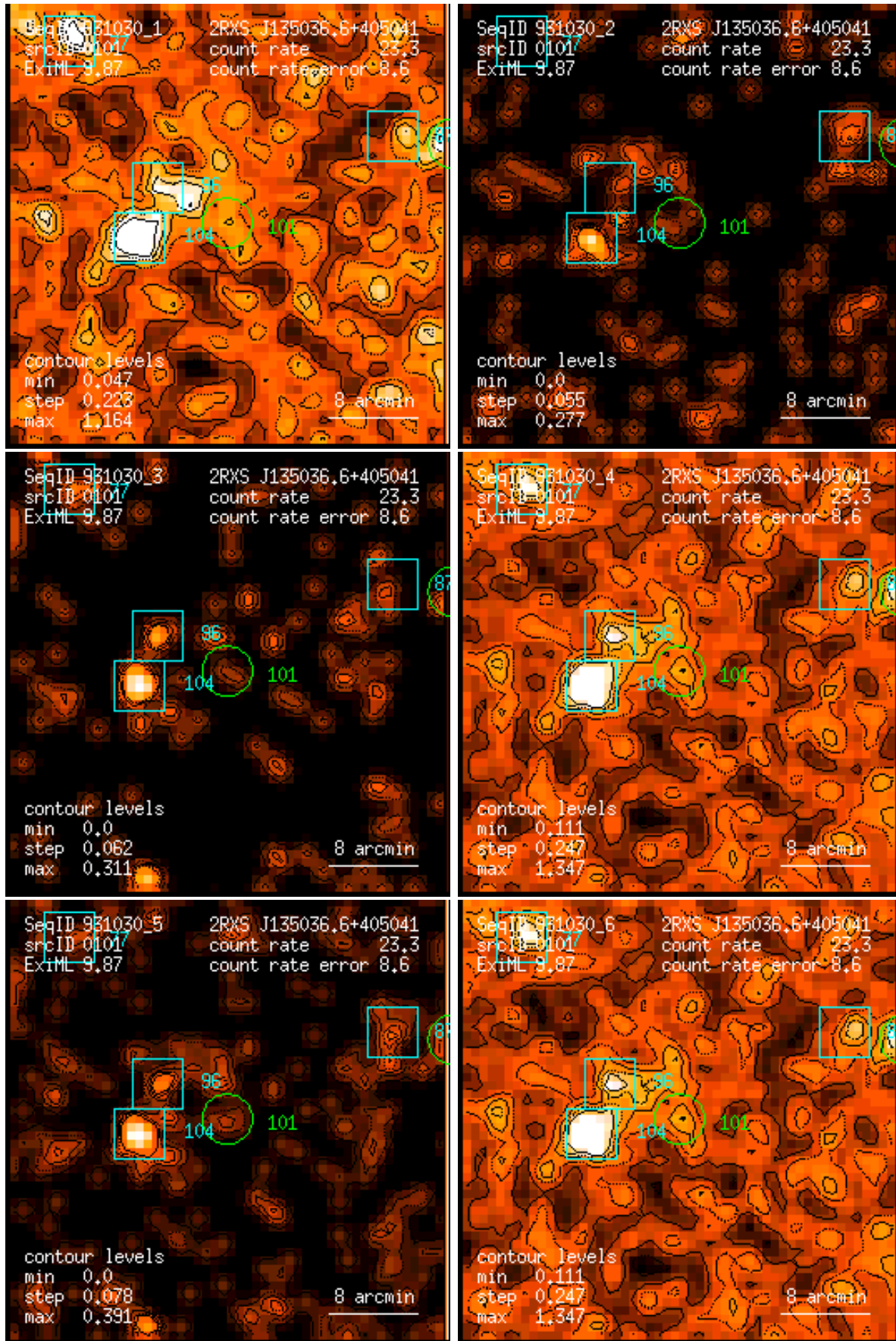
Figure 101: RASS 931030: detection 0101: band rate images, Gaussian filter: (1) PSPC channels 11 – 41, (2) 52 – 90, (3) 91 – 201, (4) 11 – 235, (5) 52 – 201, (6) 11 – 201. Broad band rates in counts/ks. Band rate contour levels in counts/ks/arcmin 2 .
