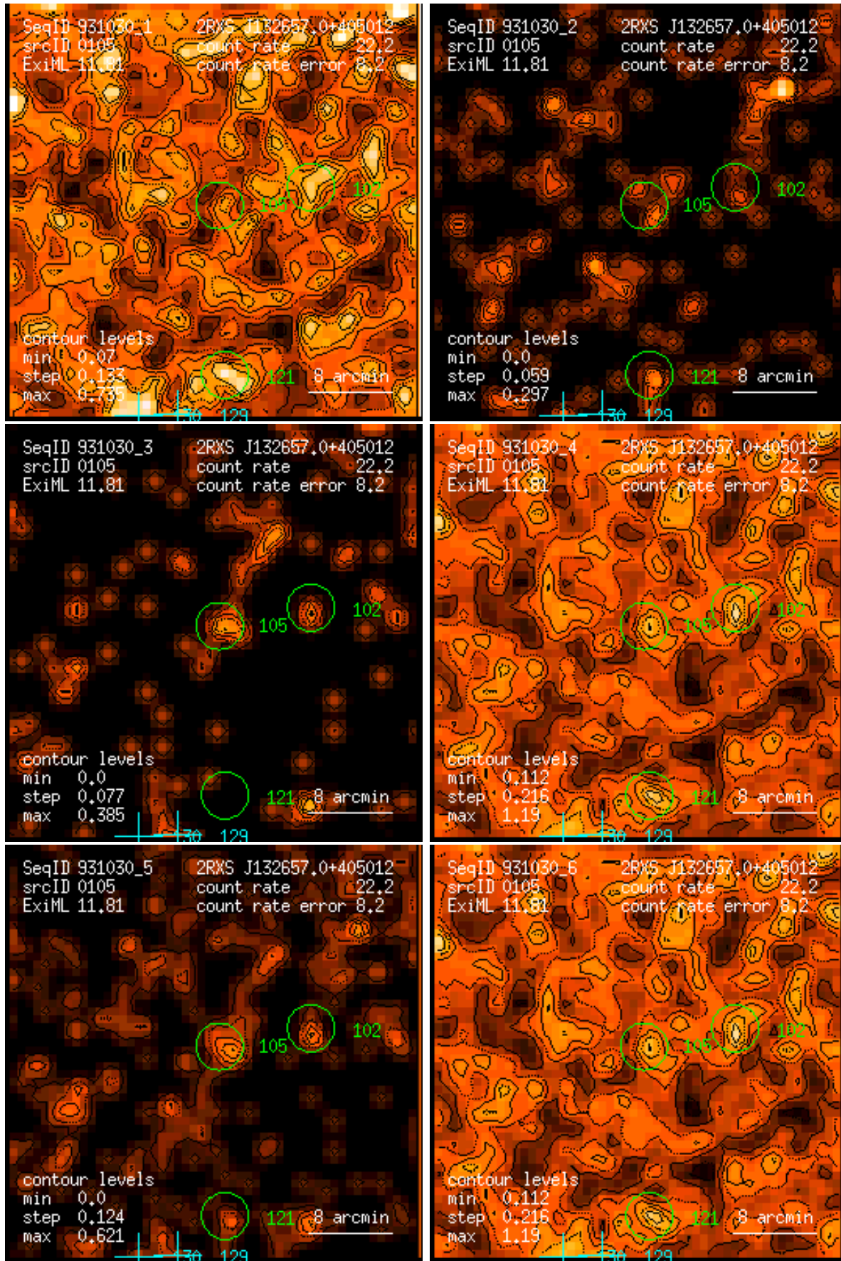
Figure 105: RASS 931030: detection 0105: band rate images, Gaussian filter: (1) PSPC channels 11 – 41, (2) 52 – 90, (3) 91 – 201, (4) 11 – 235, (5) 52 – 201, (6) 11 – 201. Broad band rates in counts/ks. Band rate contour levels in counts/ks/arcmin 2 .
