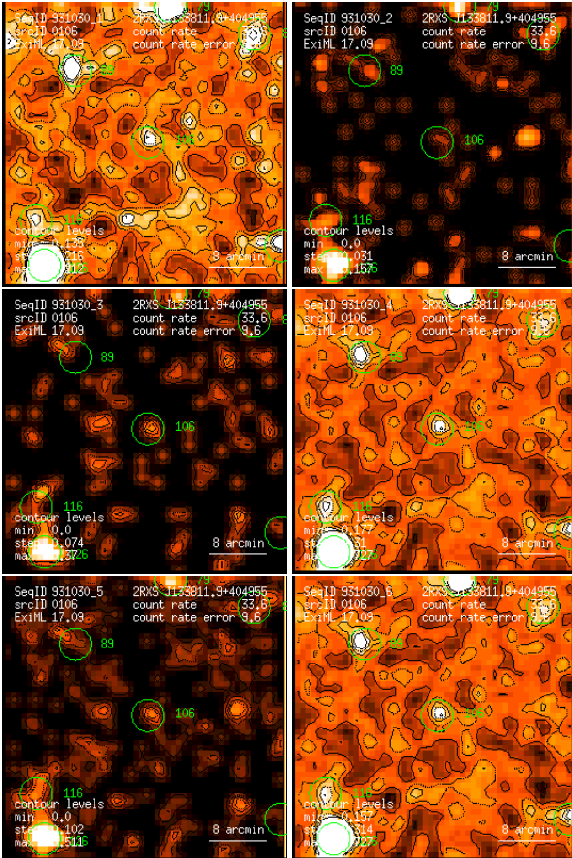
Figure 106: RASS 931030: detection 0106: band rate images, Gaussian filter: (1) PSPC channels 11 – 41, (2) 52 – 90, (3) 91 – 201, (4) 11 – 235, (5) 52 – 201, (6) 11 – 201. Broad band rates in counts/ks. Band rate contour levels in counts/ks/arcmin 2 .
