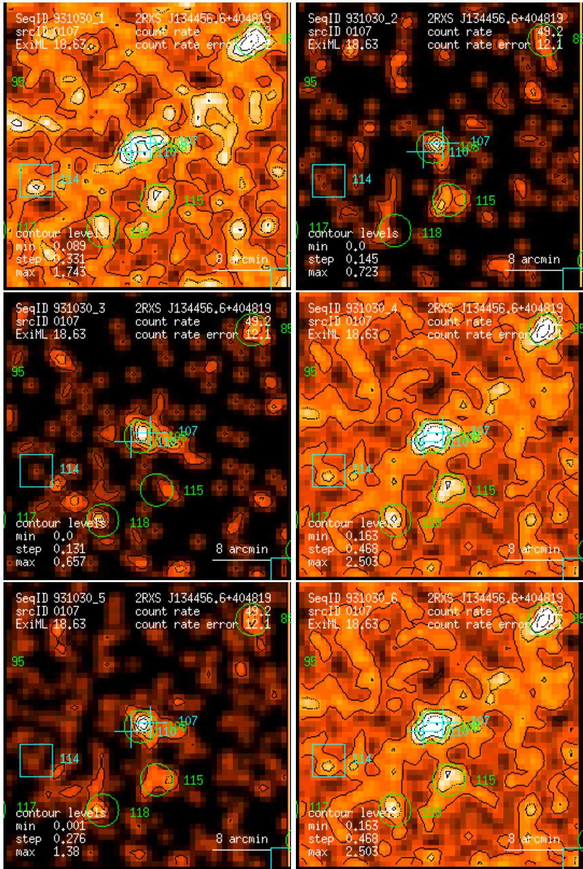
Figure 107: RASS 931030: detection 0107: band rate images, Gaussian filter: (1) PSPC channels 11 – 41, (2) 52 – 90, (3) 91 – 201, (4) 11 – 235, (5) 52 – 201, (6) 11 – 201. Broad band rates in counts/ks. Band rate contour levels in counts/ks/arcmin 2 .
