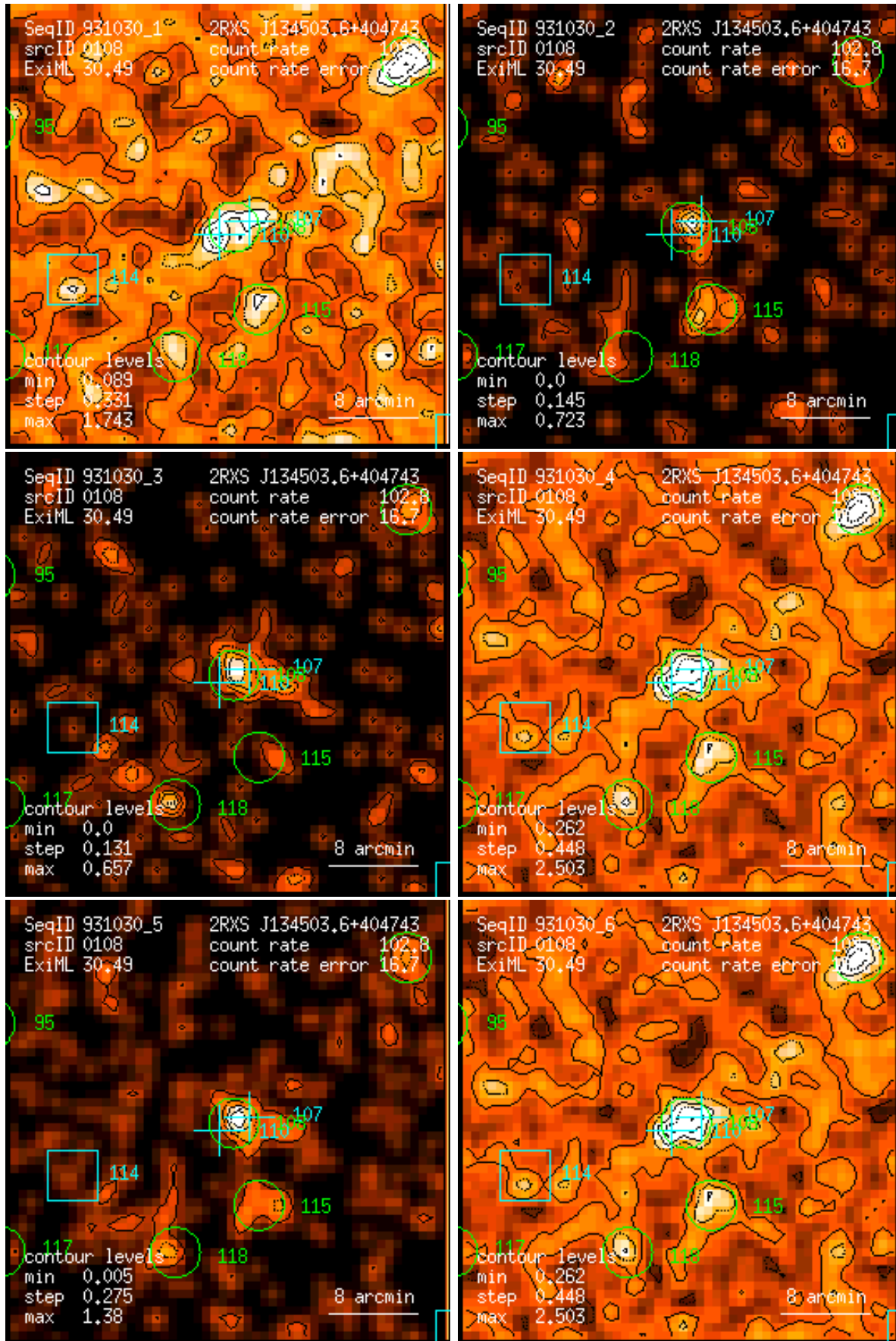
Figure 108: RASS 931030: detection 0108: band rate images, Gaussian filter: (1) PSPC channels 11 – 41, (2) 52 – 90, (3) 91 – 201, (4) 11 – 235, (5) 52 – 201, (6) 11 – 201. Broad band rates in counts/ks. Band rate contour levels in counts/ks/arcmin 2 .
