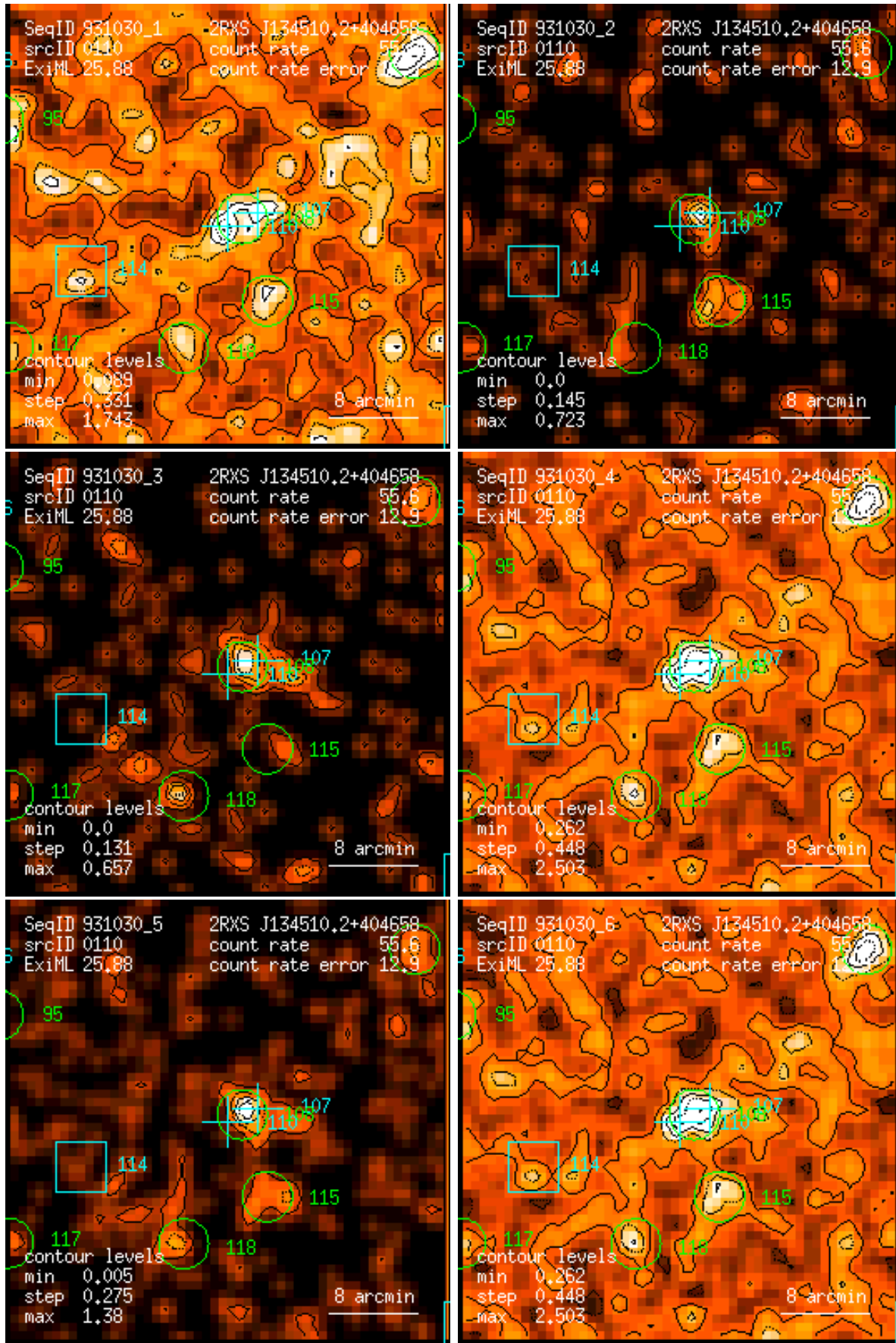
Figure 110: RASS 931030: detection 0110: band rate images, Gaussian filter: (1) PSPC channels 11 – 41, (2) 52 – 90, (3) 91 – 201, (4) 11 – 235, (5) 52 – 201, (6) 11 – 201. Broad band rates in counts/ks. Band rate contour levels in counts/ks/arcmin 2 .
