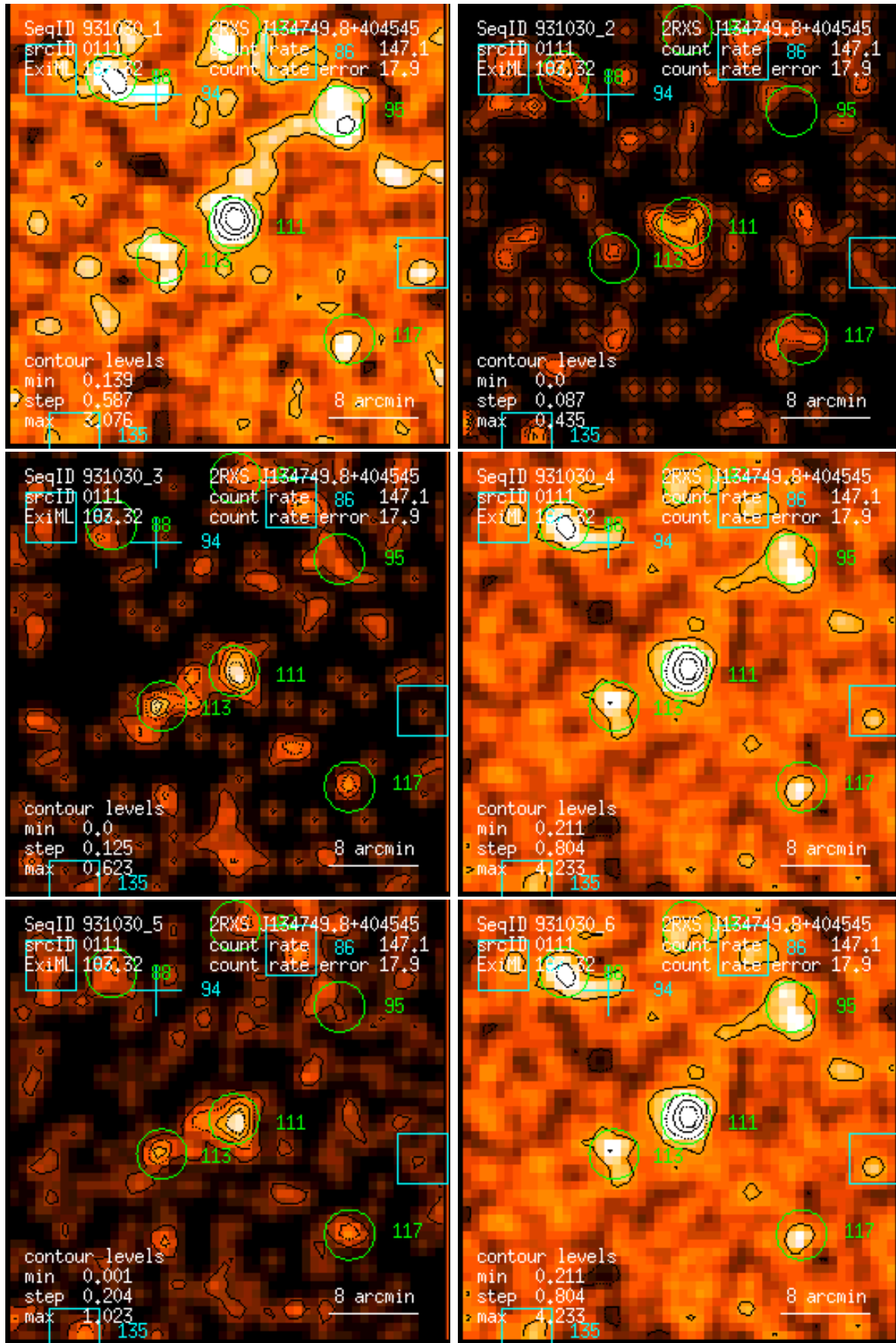
Figure 111: RASS 931030: detection 0111: band rate images, Gaussian filter: (1) PSPC channels 11 – 41, (2) 52 – 90, (3) 91 – 201, (4) 11 – 235, (5) 52 – 201, (6) 11 – 201. Broad band rates in counts/ks. Band rate contour levels in counts/ks/arcmin 2 .
