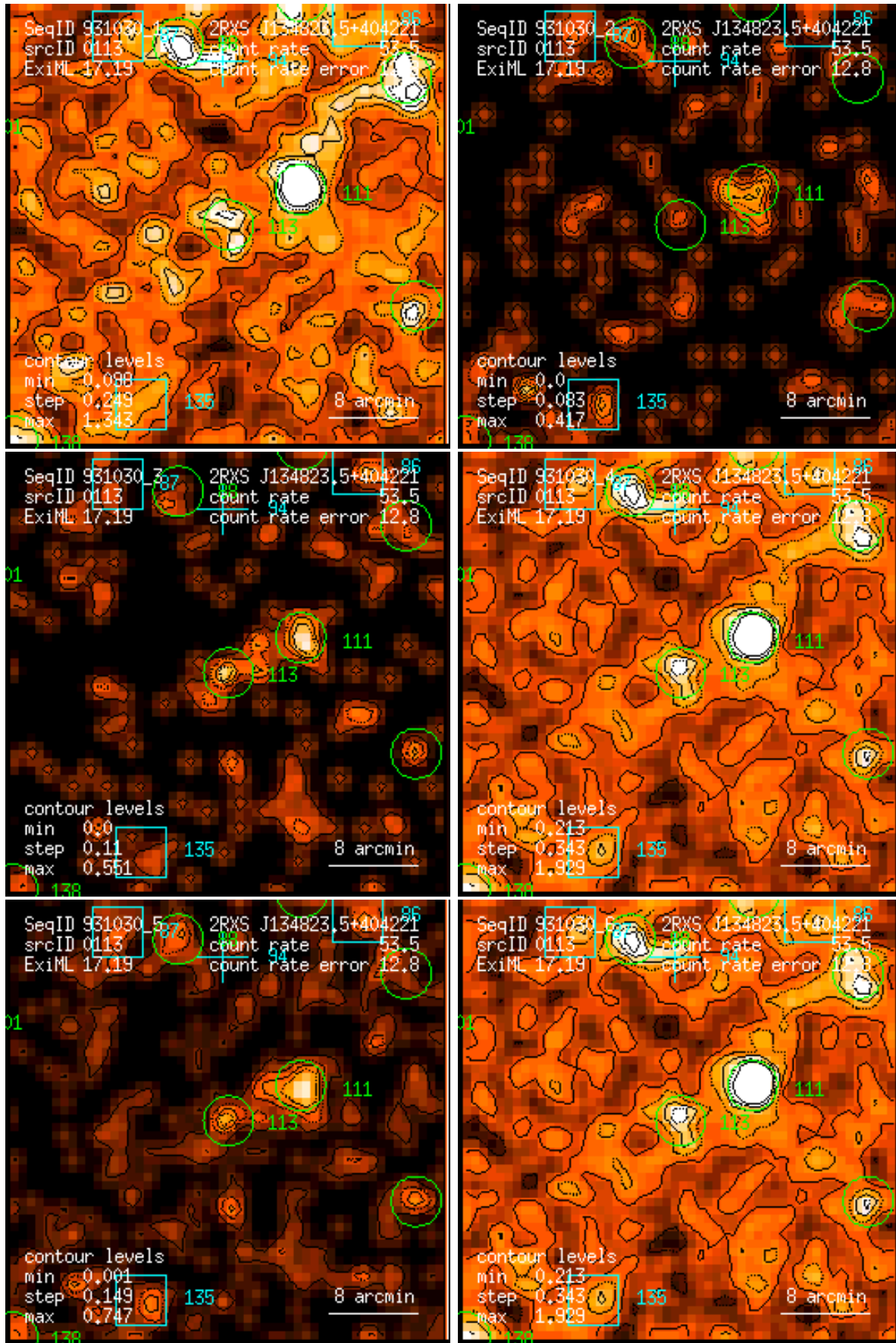
Figure 113: RASS 931030: detection 0113: band rate images, Gaussian filter: (1) PSPC channels 11 – 41, (2) 52 – 90, (3) 91 – 201, (4) 11 – 235, (5) 52 – 201, (6) 11 – 201. Broad band rates in counts/ks. Band rate contour levels in counts/ks/arcmin 2 .
