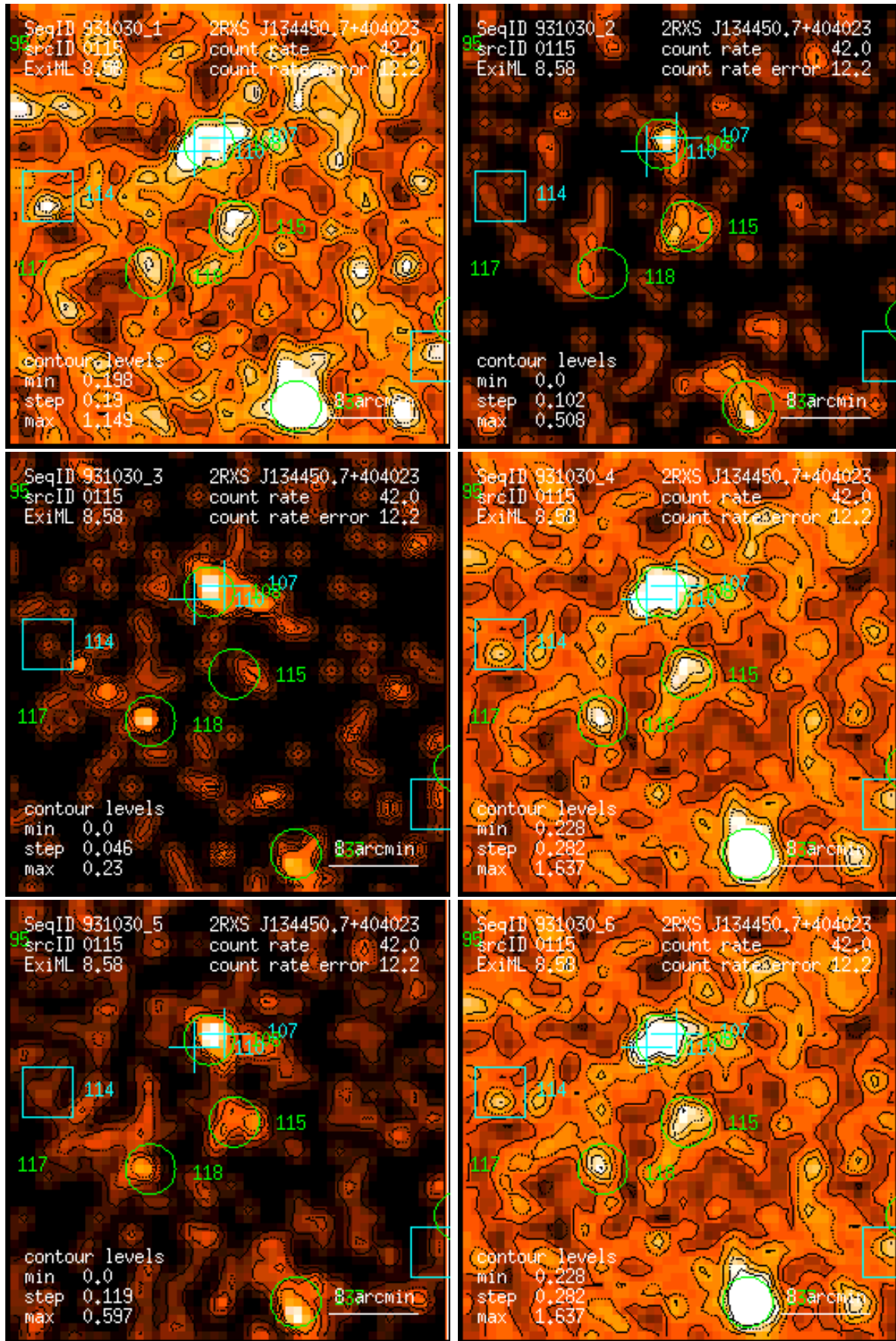
Figure 115: RASS 931030: detection 0115: band rate images, Gaussian filter: (1) PSPC channels 11 – 41, (2) 52 – 90, (3) 91 – 201, (4) 11 – 235, (5) 52 – 201, (6) 11 – 201. Broad band rates in counts/ks. Band rate contour levels in counts/ks/arcmin 2 .
