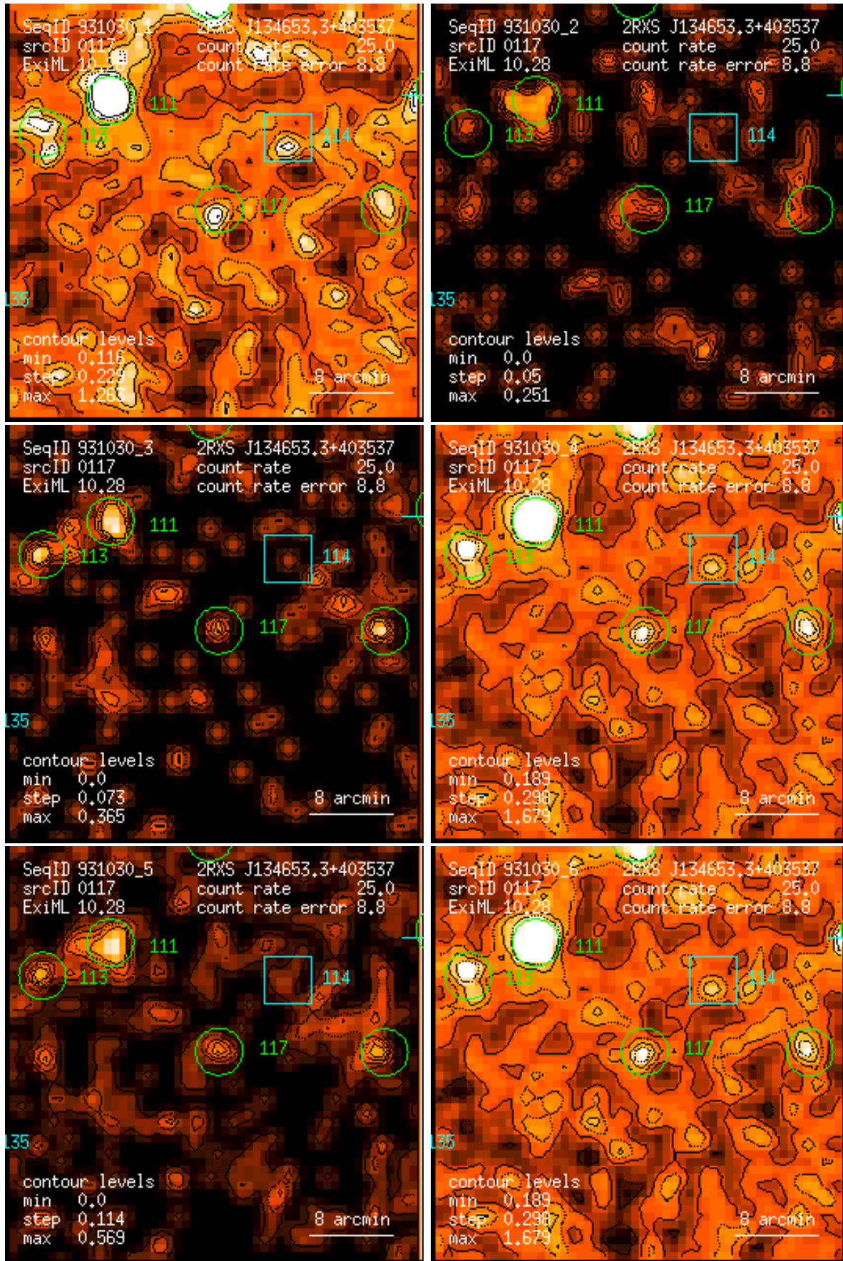
Figure 117: RASS 931030: detection 0117: band rate images, Gaussian filter: (1) PSPC channels 11 – 41, (2) 52 – 90, (3) 91 – 201, (4) 11 – 235, (5) 52 – 201, (6) 11 – 201. Broad band rates in counts/ks. Band rate contour levels in counts/ks/arcmin 2 .
