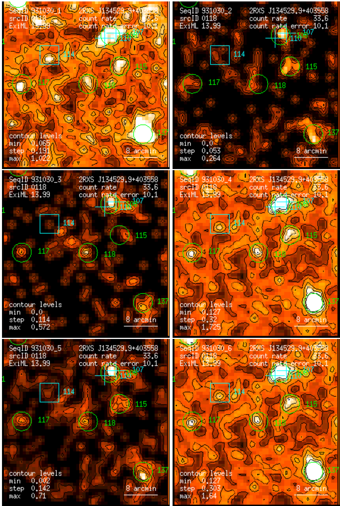
Figure 118: RASS 931030: detection 0118: band rate images, Gaussian filter: (1) PSPC channels 11 – 41, (2) 52 – 90, (3) 91 – 201, (4) 11 – 235, (5) 52 – 201, (6) 11 – 201. Broad band rates in counts/ks. Band rate contour levels in counts/ks/arcmin 2 .
