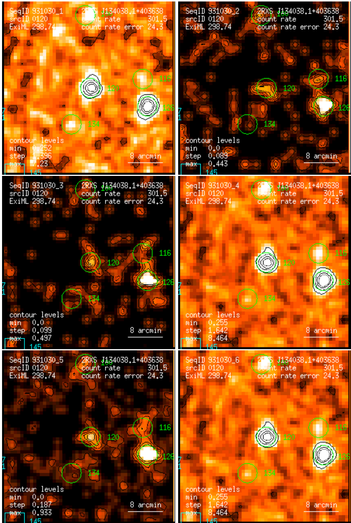
Figure 120: RASS 931030: detection 0120: band rate images, Gaussian filter: (1) PSPC channels 11 – 41, (2) 52 – 90, (3) 91 – 201, (4) 11 – 235, (5) 52 – 201, (6) 11 – 201. Broad band rates in counts/ks. Band rate contour levels in counts/ks/arcmin 2 .
