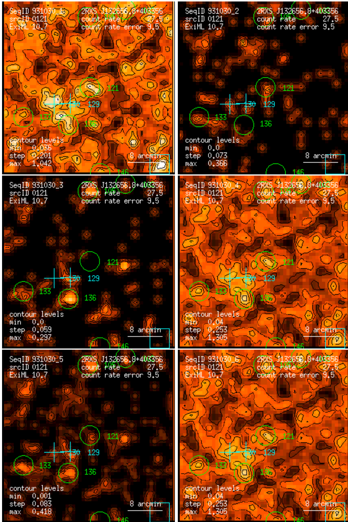
Figure 121: RASS 931030: detection 0121: band rate images, Gaussian filter: (1) PSPC channels 11 – 41, (2) 52 – 90, (3) 91 – 201, (4) 11 – 235, (5) 52 – 201, (6) 11 – 201. Broad band rates in counts/ks. Band rate contour levels in counts/ks/arcmin 2 .
