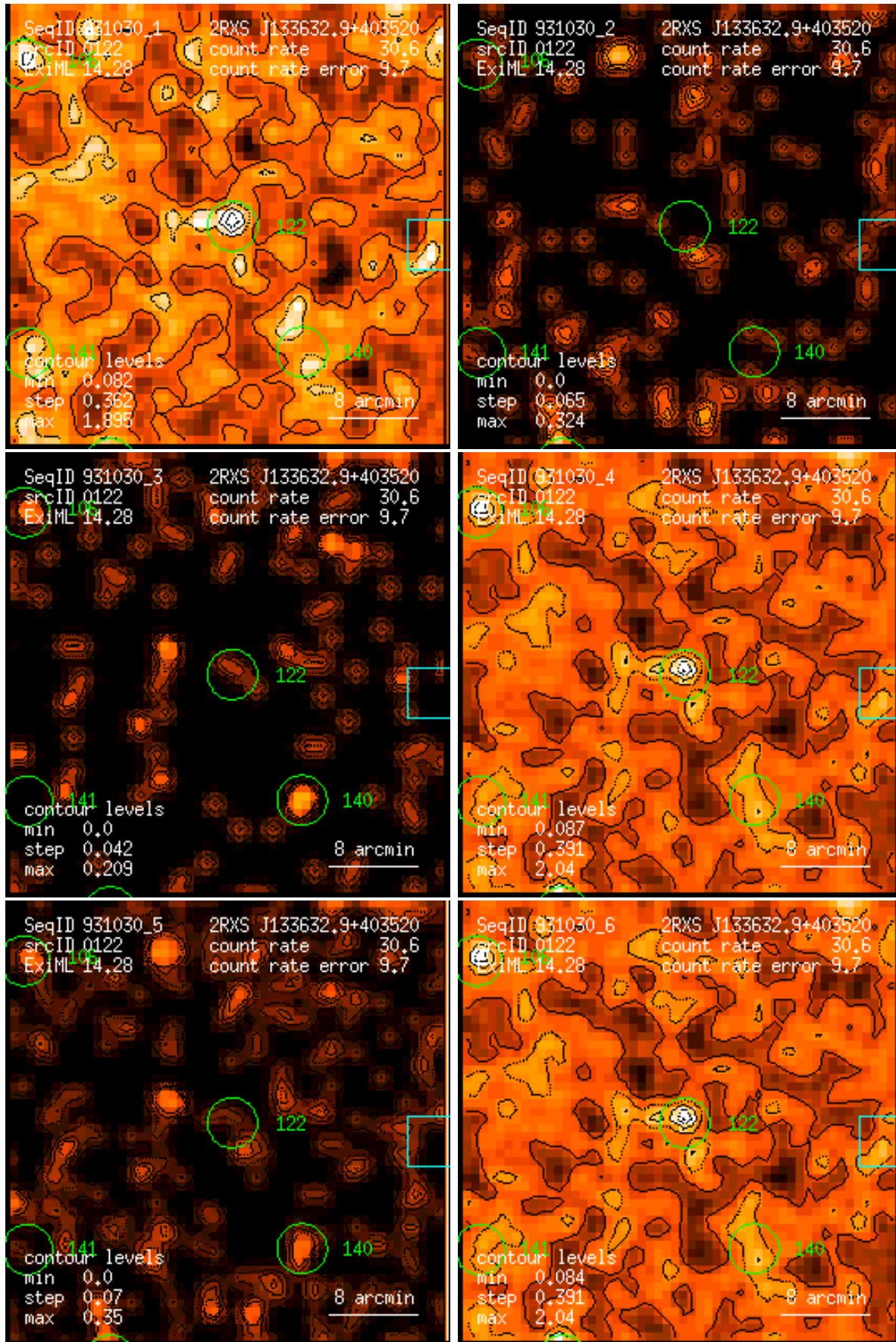
Figure 122: RASS 931030: detection 0122: band rate images, Gaussian filter: (1) PSPC channels 11 – 41, (2) 52 – 90, (3) 91 – 201, (4) 11 – 235, (5) 52 – 201, (6) 11 – 201. Broad band rates in counts/ks. Band rate contour levels in counts/ks/arcmin 2 .
