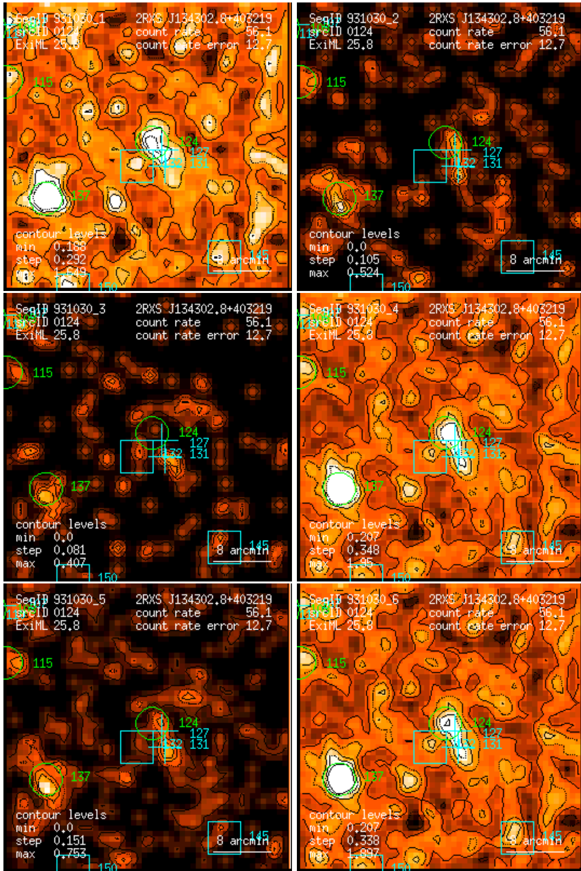
Figure 124: RASS 931030: detection 0124: band rate images, Gaussian filter: (1) PSPC channels 11 – 41, (2) 52 – 90, (3) 91 – 201, (4) 11 – 235, (5) 52 – 201, (6) 11 – 201. Broad band rates in counts/ks. Band rate contour levels in counts/ks/arcmin 2 .
