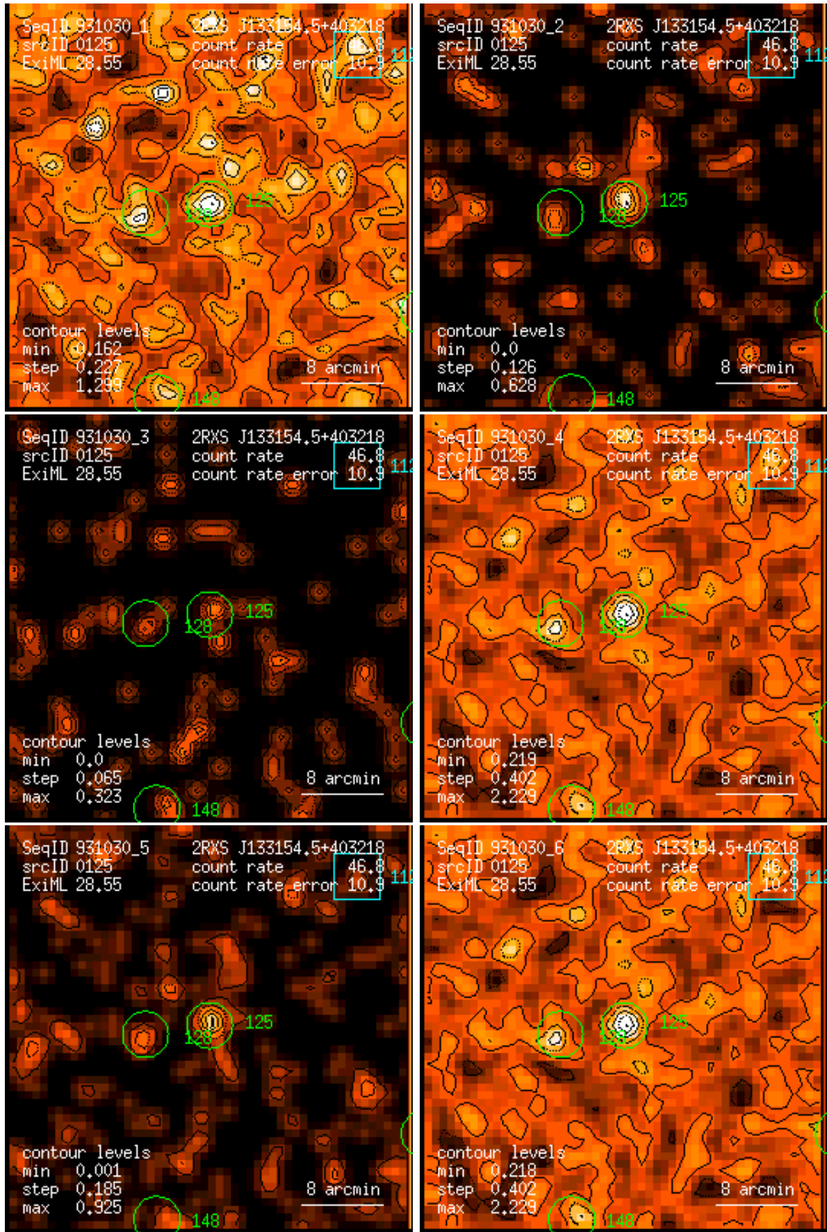
Figure 125: RASS 931030: detection 0125: band rate images, Gaussian filter: (1) PSPC channels 11 – 41, (2) 52 – 90, (3) 91 – 201, (4) 11 – 235, (5) 52 – 201, (6) 11 – 201. Broad band rates in counts/ks. Band rate contour levels in counts/ks/arcmin 2 .
