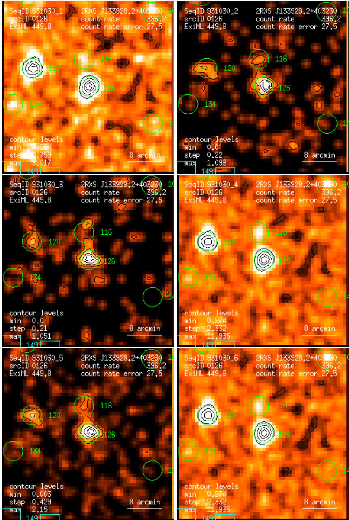
Figure 126: RASS 931030: detection 0126: band rate images, Gaussian filter: (1) PSPC channels 11 – 41, (2) 52 – 90, (3) 91 – 201, (4) 11 – 235, (5) 52 – 201, (6) 11 – 201. Broad band rates in counts/ks. Band rate contour levels in counts/ks/arcmin 2 .
