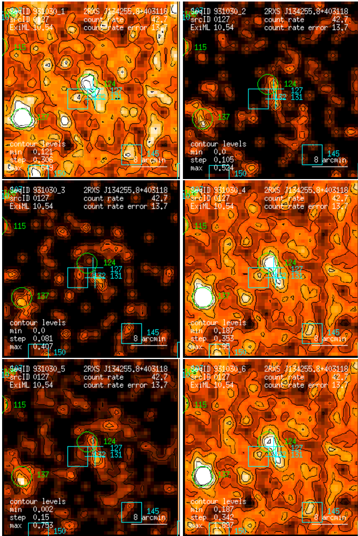
Figure 127: RASS 931030: detection 0127: band rate images, Gaussian filter: (1) PSPC channels 11 – 41, (2) 52 – 90, (3) 91 – 201, (4) 11 – 235, (5) 52 – 201, (6) 11 – 201. Broad band rates in counts/ks. Band rate contour levels in counts/ks/arcmin 2 .
