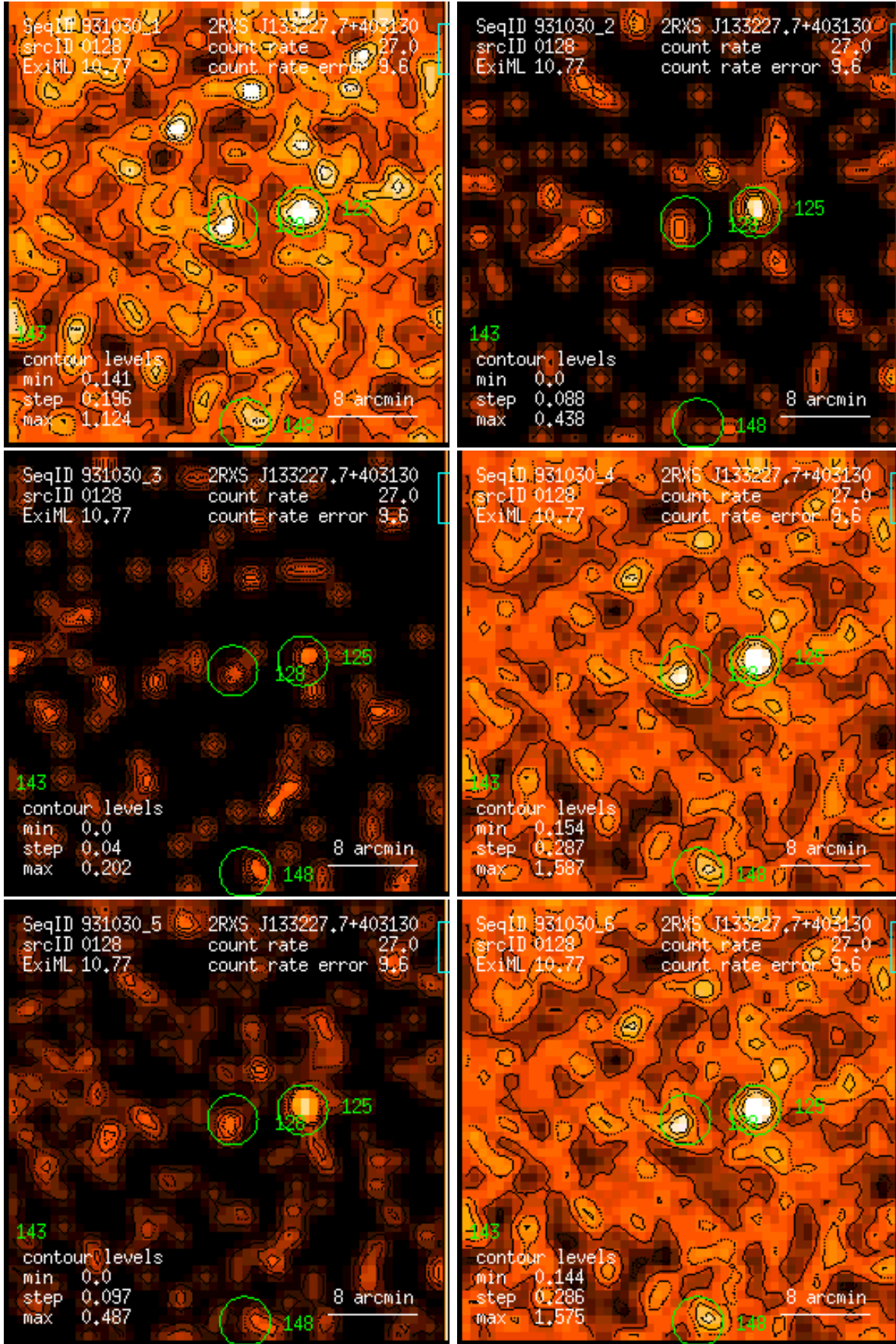
Figure 128: RASS 931030: detection 0128: band rate images, Gaussian filter: (1) PSPC channels 11 – 41, (2) 52 – 90, (3) 91 – 201, (4) 11 – 235, (5) 52 – 201, (6) 11 – 201. Broad band rates in counts/ks. Band rate contour levels in counts/ks/arcmin 2 .
