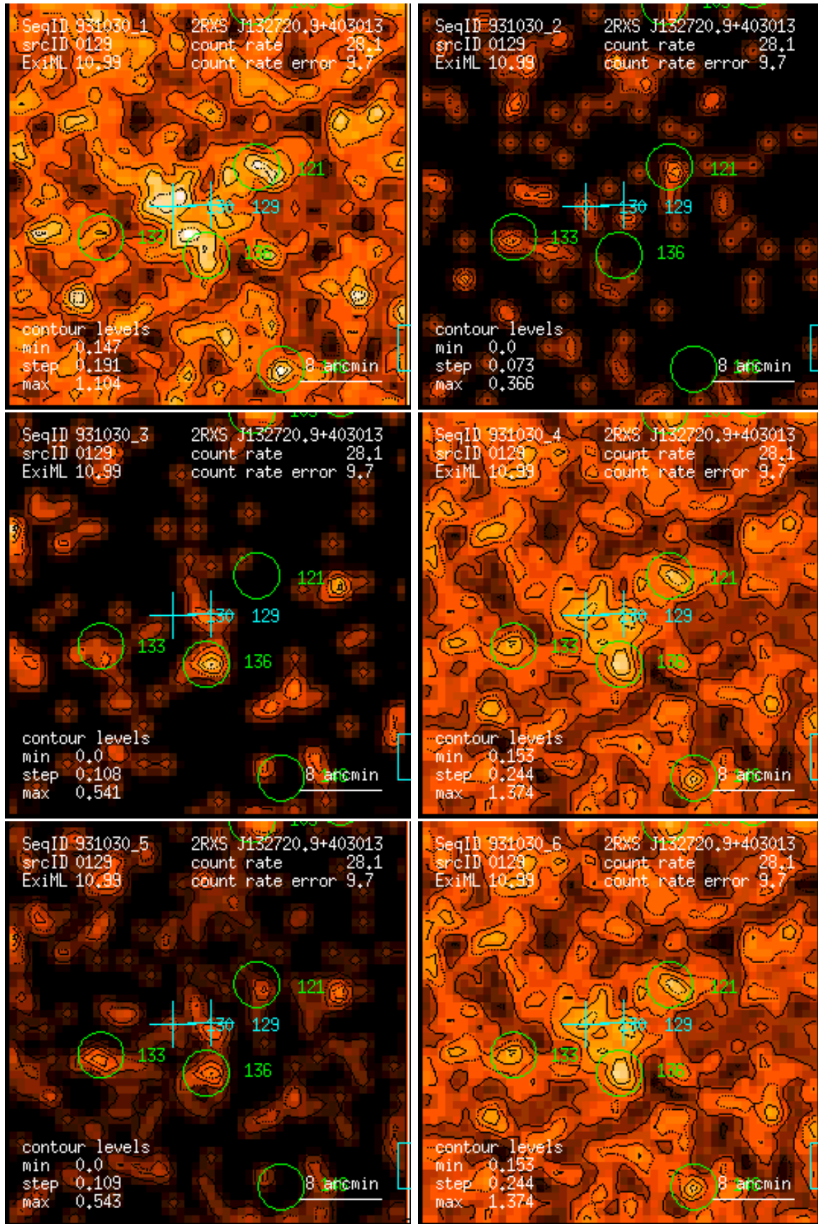
Figure 129: RASS 931030: detection 0129: band rate images, Gaussian filter: (1) PSPC channels 11 – 41, (2) 52 – 90, (3) 91 – 201, (4) 11 – 235, (5) 52 – 201, (6) 11 – 201. Broad band rates in counts/ks. Band rate contour levels in counts/ks/arcmin 2 .
