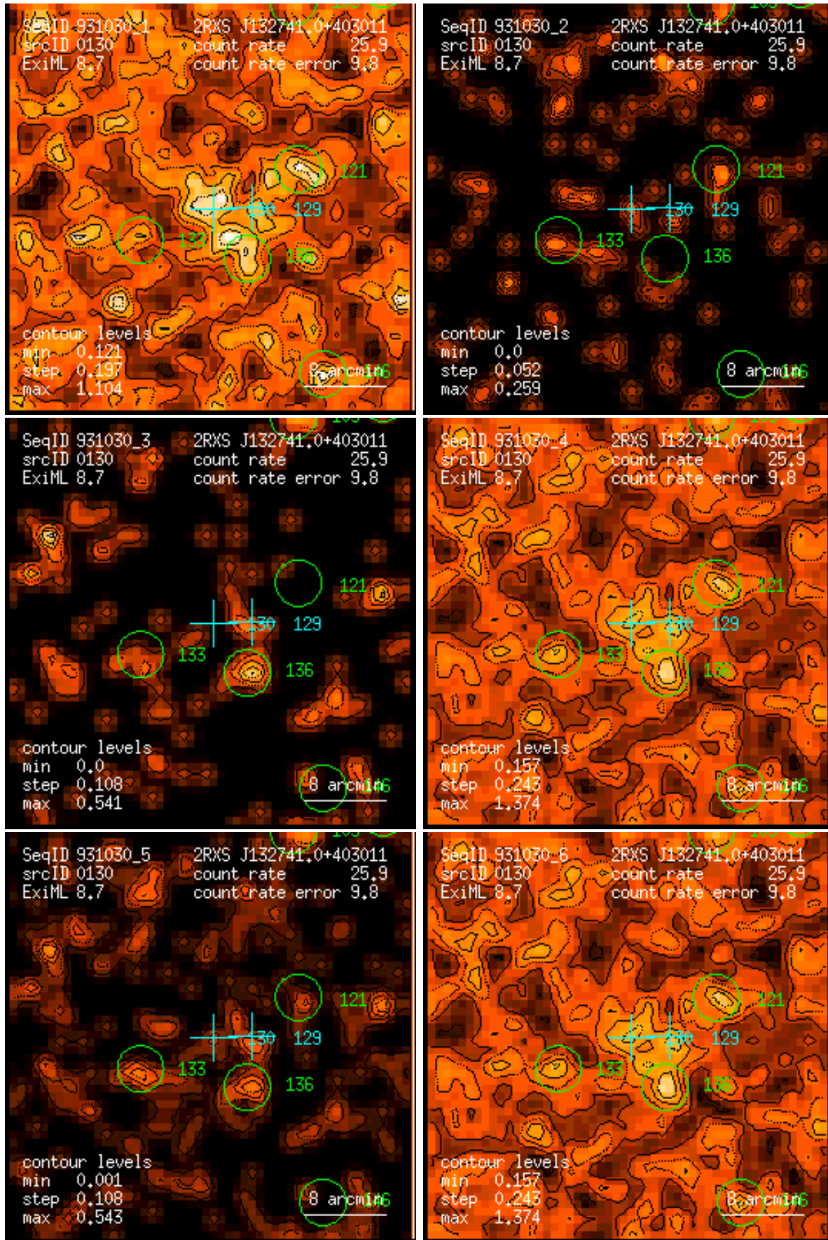
Figure 130: RASS 931030: detection 0130: band rate images, Gaussian filter: (1) PSPC channels 11 – 41, (2) 52 – 90, (3) 91 – 201, (4) 11 – 235, (5) 52 – 201, (6) 11 – 201. Broad band rates in counts/ks. Band rate contour levels in counts/ks/arcmin 2 .
